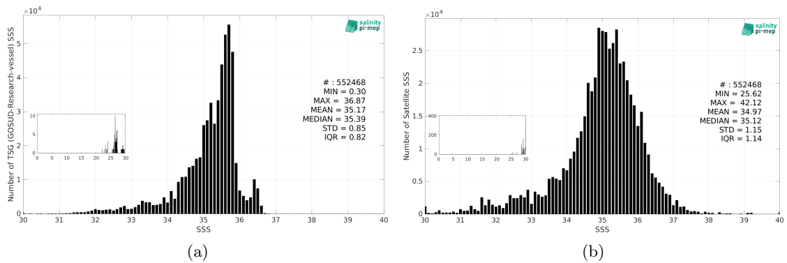
Figure 3: Histograms of SSS from TSG (GOSUD-Research-vessel) (a) and SMAP SSS L2 v5.0 (JPL) (b) considering all match-up pairs per bins of 0.1 over the Pacific Ocean Pi-MEP region and for the full satellite product period.
