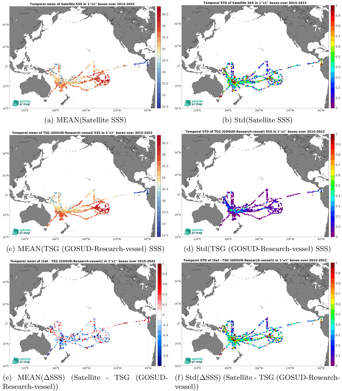
Figure 7: Temporal mean (left) and Std (right) of SSS from SMAP SSS L2 v5.0 (JPL) (top), TSG (GOSUD-Research-vessel) (middle), and of \Delta SSS (Satellite - TSG (GOSUD-Research-vessel)). Only match-up pairs are used to generate these maps.
