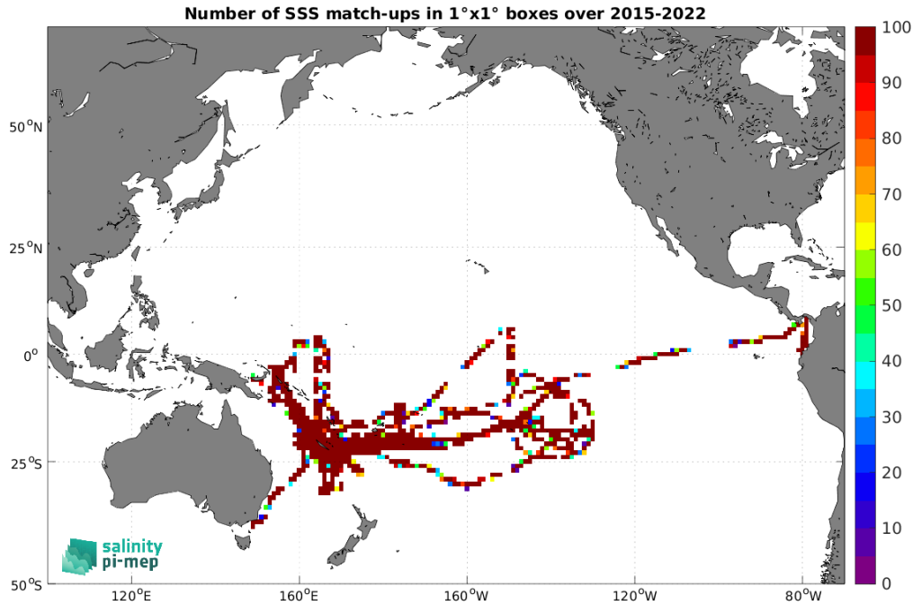
Figure 5: Number of SSS match-ups between TSG (GOSUD-Research-vessel) SSS and the SMAP SSS L2 v5.0 (JPL) SSS product for the Pacific Ocean Pi-MEP region over 1°x1° boxes and for the full satellite product period.
