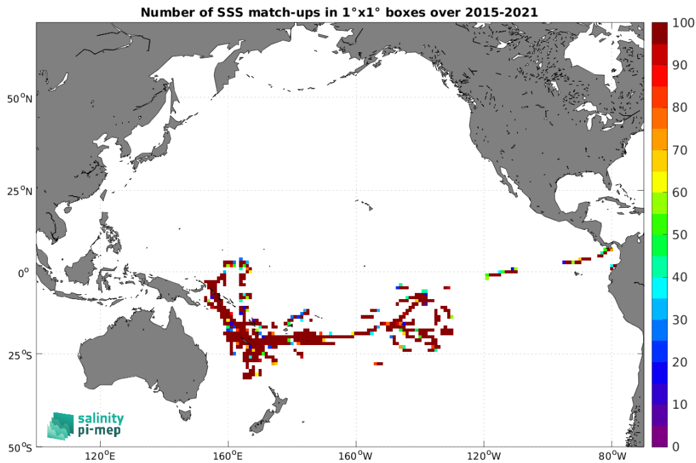
Figure 5: Number of SSS match-ups between TSG (GOSUD-Research-vessel) SSS and the SMAP SSS L2 v5.0 (JPL) SSS product for the Pacific Ocean Pi-MEP region over 1^\circ \times 1^\circ boxes and for the full satellite product period.
