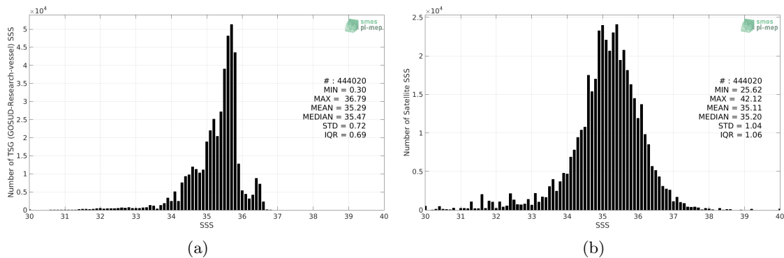
Figure 2: Histograms of SSS from TSG (GOSUD-Research-vessel) (a) and SMAP SSS L2 v5.0 (JPL) (b) considering all match-up pairs per bins of 0.1 over the Pacific Ocean Pi-MEP region and for the full satellite product period.
