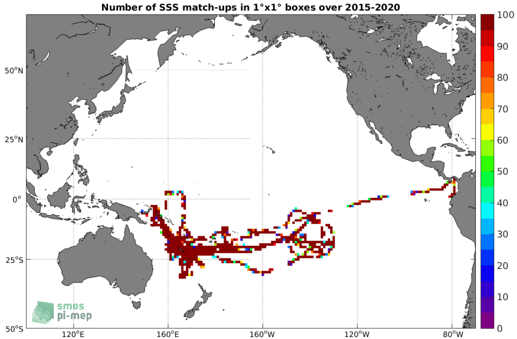
Figure 4: Number of SSS match-ups between TSG (GOSUD-Research-vessel) SSS and the SMAP SSS L2 v5.0 (JPL) SSS product for the Pacific Ocean Pi-MEP region over 1^\circ \times 1^\circ boxes and for the full satellite product period.
