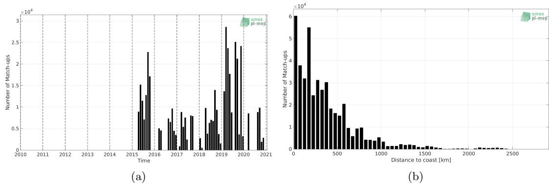
Figure 1: Number of match-ups between TSG (GOSUD-Research-vessel) and SMAP SSS L2 v5.0 (JPL) SSS as a function of time (a) and as function of the distance to coast (b) over the Pacific Ocean Pi-MEP region and for the full satellite product period.
