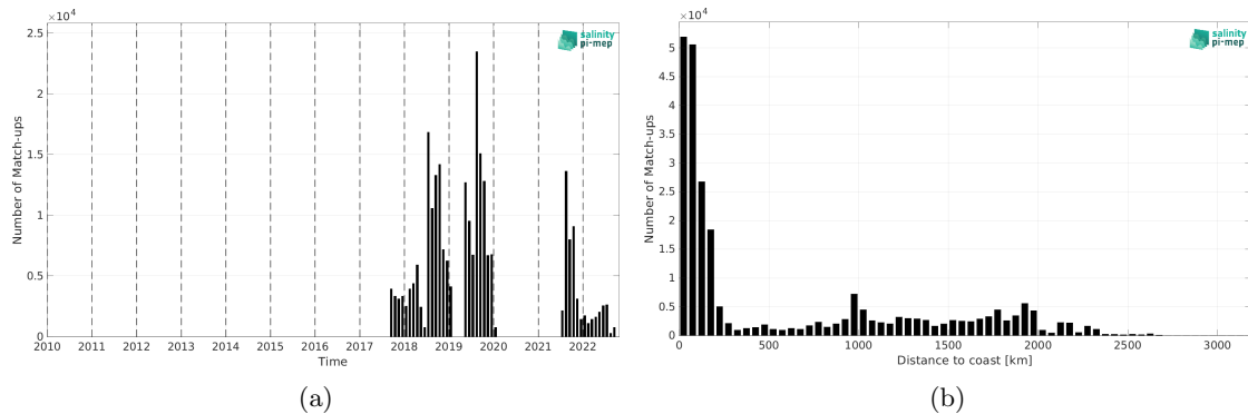
Figure 2: Number of match-ups between Sairdrone and SMAP SSS L2 v5.0 (JPL) SSS as a function of time (a) and as function of the distance to coast (b) over the Pacific Ocean Pi-MEP region and for the full satellite product period.
