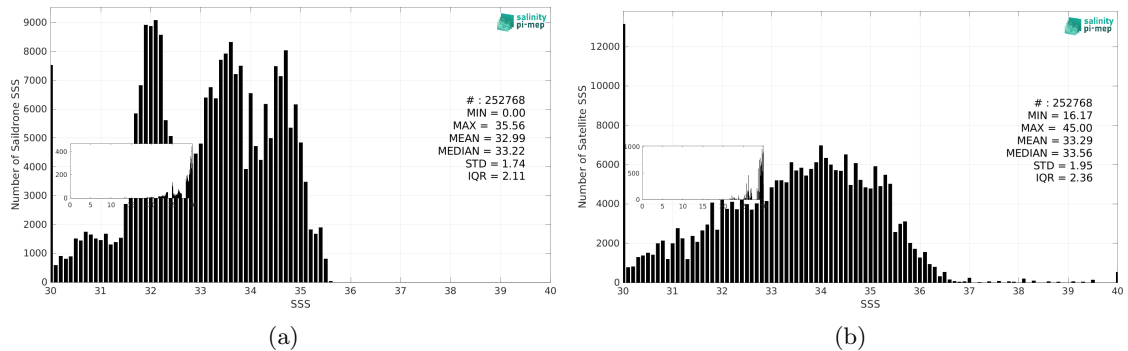
Figure 3: Histograms of SSS from Sairdrone (a) and SMAP SSS L2 v5.0 (JPL) (b) considering all match-up pairs per bins of 0.1 over the Pacific Ocean Pi-MEP region and for the full satellite product period.
