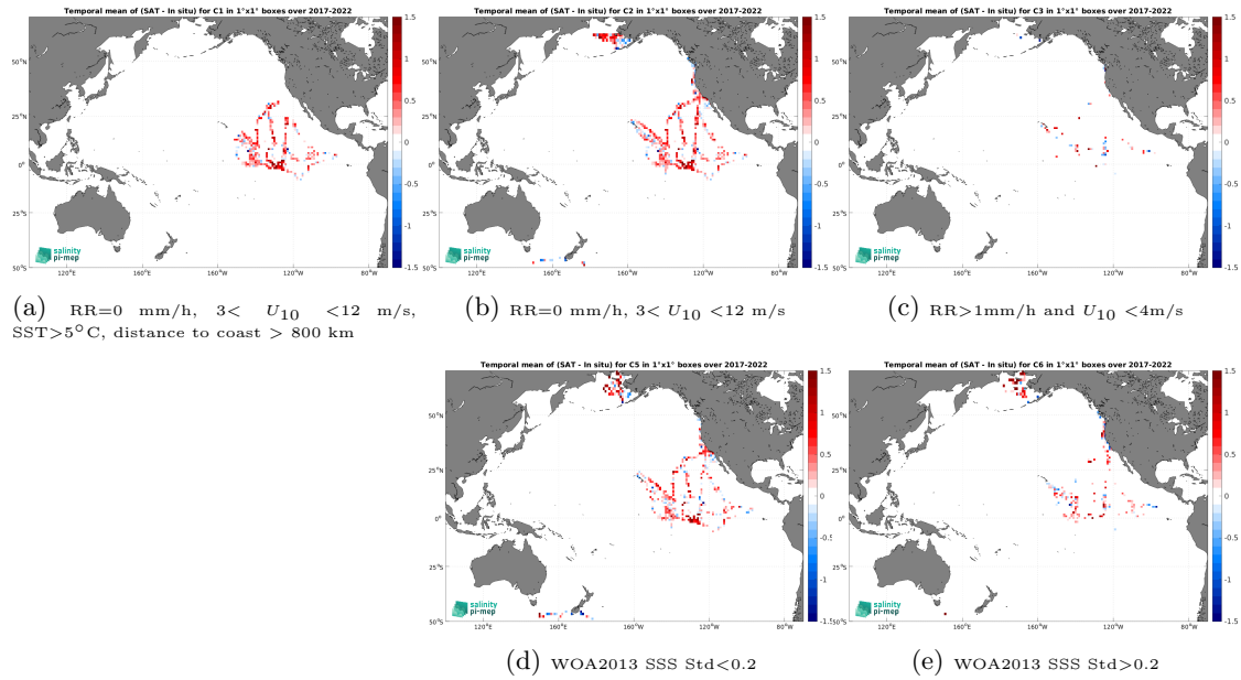
Figure 12: Temporal mean gridded over spatial boxes of size 1^\circ \times 1^\circ of \Delta SSS (SMAP SSS L2 v5.0 (JPL) - Saifdrone) for 5 different subdatasets corresponding to:RR=0 mm/h, 3 < U_{10} < 12 m/s, SST >5^\circ C, distance to coast > 800 km (a), RR=0 mm/h, 3 < U_{10} < 12 m/s (b), RR >1 mm/h and U_{10} < 4 m/s (c), WOA2013 SSS Std <0.2 (d), WOA2013 SSS Std >0.2 (e).
