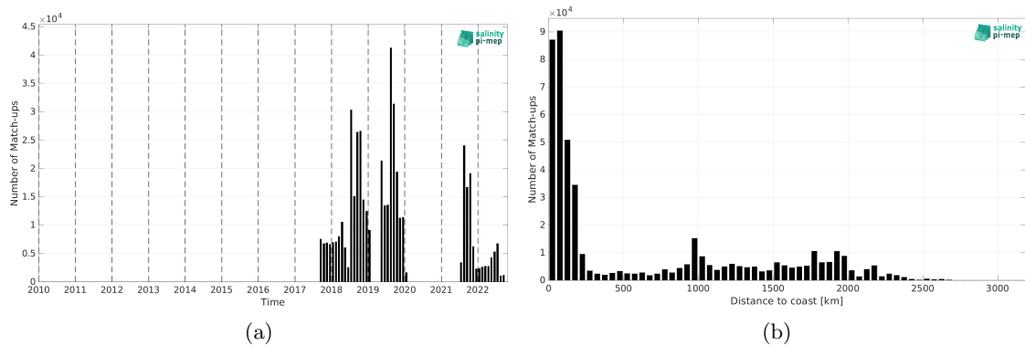
Figure 1: Number of match-ups between Sairdrone and SMAP SSS L2 v5.0 (JPL) SSS as a function of time (a) and as function of the distance to coast (b) over the Pacific Ocean Pi-MEP region and for the full satellite product period.
