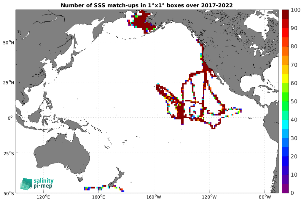
Figure 4: Number of SSS match-ups between Saildrone SSS and the SMAP SSS L2 v5.0 (JPL) SSS product for the Pacific Ocean Pi-MEP region over 1^\circ \times 1^\circ boxes and for the full satellite product period.
