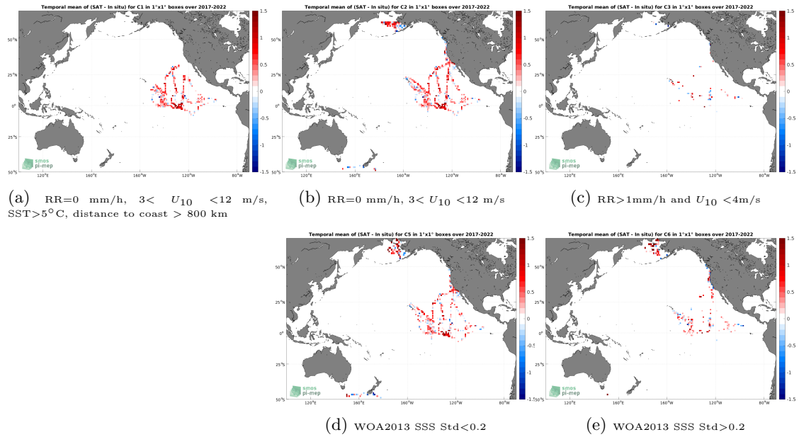
Figure 12: Temporal mean gridded over spatial boxes of size 1^\circ \times 1^\circ of \Delta SSS (SMAP SSS L2 v5.0 (JPL) - Saikrone) for 5 different subdatasets corresponding to:RR=0 mm/h, 3 < U_{10} < 12 m/s, SST >5^\circ C, distance to coast > 800 km (a), RR=0 mm/h, 3 < U_{10} < 12 m/s (b), RR >1 mm/h and U_{10} < 4 m/s (c), WOA2013 SSS Std <0.2 (d), WOA2013 SSS Std >0.2 (e).
