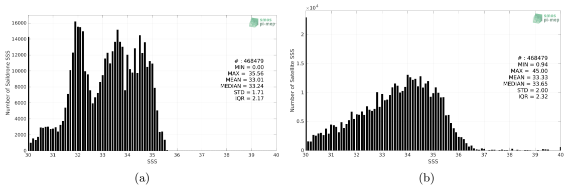
Figure 2: Histograms of SSS from Sairdron (a) and SMAP SSS L2 v5.0 (JPL) (b) considering all match-up pairs per bins of 0.1 over the Pacific Ocean Pi-MEP region and for the full satellite product period.
