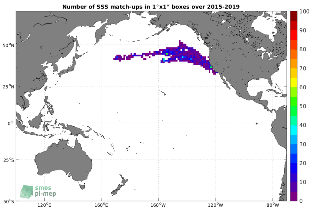
Figure 4: Number of SSS match-ups between Marine mammals SSS and the SMAP SSS L2 v5.0 (JPL) SSS product for the Pacific Ocean Pi-MEP region over 1^\circ \times 1^\circ boxes and for the full satellite product period.
