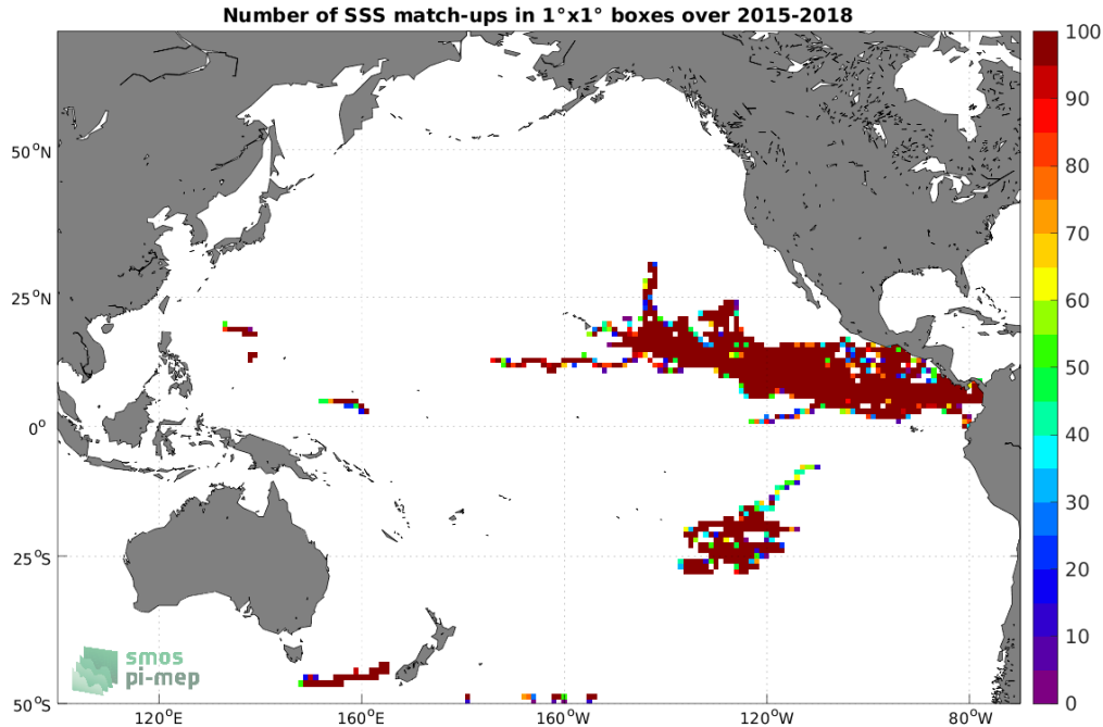
Figure 3: Number of SSS match-ups between Surface drifters SSS and the SMAP SSS L2 v5.0 (JPL) SSS product for the Pacific Ocean Pi-MEP region over 1^\circ \times 1^\circ boxes and for the full satellite product period.
