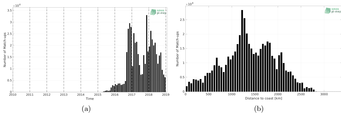
Figure 1: Number of match-ups between Surface drifters and SMAP SSS L2 v5.0 (JPL) SSS as a function of time (a) and as function of the distance to coast (b) over the Pacific Ocean Pi-MEP region and for the full satellite product period.
