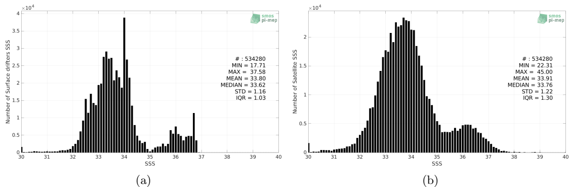
Figure 2: Histograms of SSS from Surface drifters (a) and SMAP SSS L2 v5.0 (JPL) (b) considering all match-up pairs per bins of 0.1 over the Pacific Ocean Pi-MEP region and for the full satellite product period.
