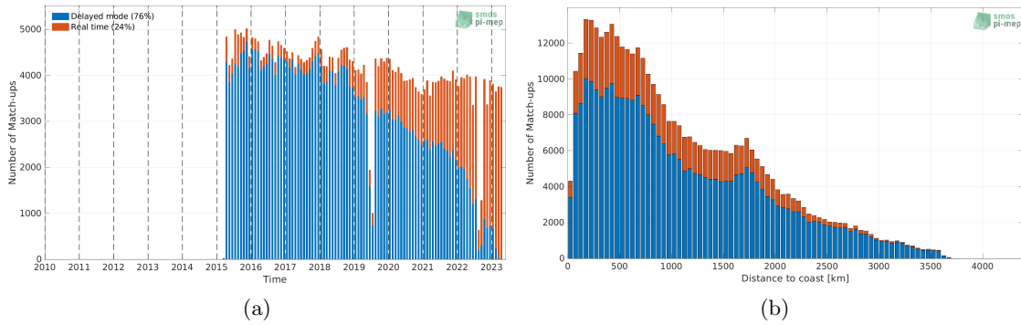
Figure 1: Number of match-ups between Argo and SMAP SSS L2 v5.0 (JPL) SSS as a function of time (a) and as function of the distance to coast (b) over the Pacific Ocean Pi-MEP region and for the full satellite product period.
