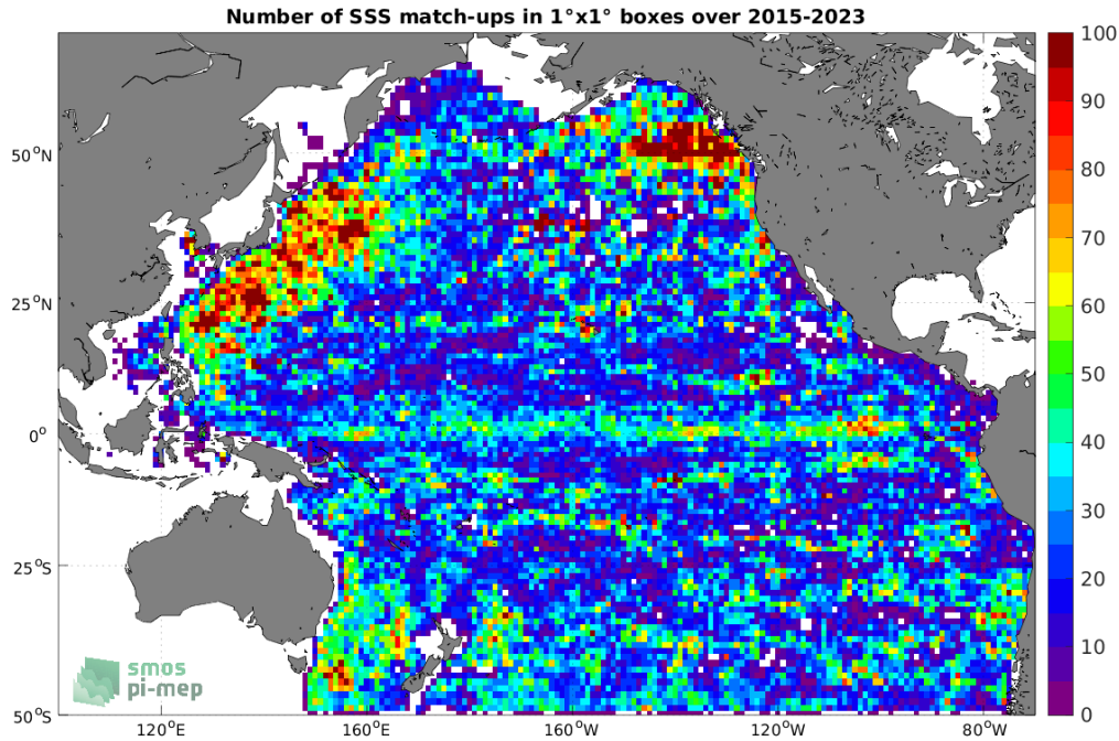
Figure 4: Number of SSS match-ups between Argo SSS and the SMAP SSS L2 v5.0 (JPL) SSS product for the Pacific Ocean Pi-MEP region over 1^\circ \times 1^\circ boxes and for the full satellite product period.
