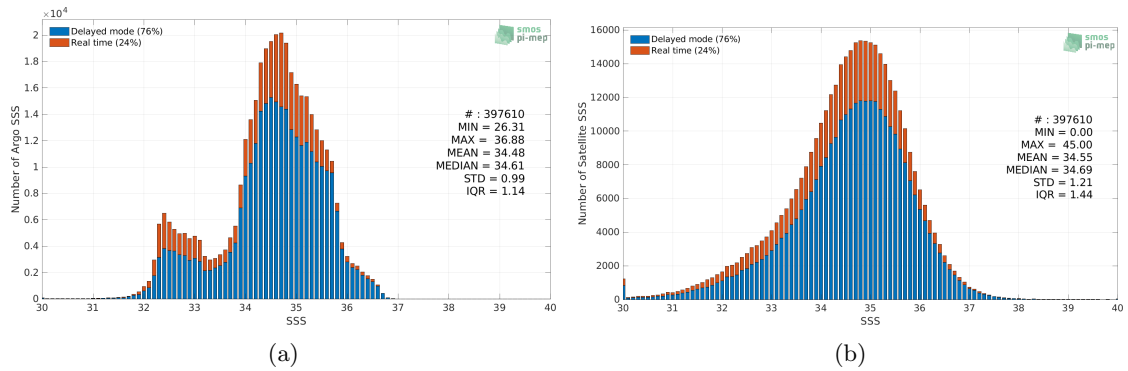
Figure 2: Histograms of SSS from Argo (a) and SMAP SSS L2 v5.0 (JPL) (b) considering all match-up pairs per bins of 0.1 over the Pacific Ocean Pi-MEP region and for the full satellite product period.
