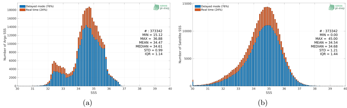
Figure 2: Histograms of SSS from Argo (a) and SMAP SSS L2 v5.0 (JPL) (b) considering all match-up pairs per bins of 0.1 over the Pacific Ocean Pi-MEP region and for the full satellite product period.
