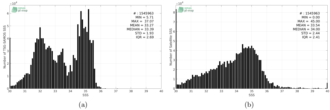
Figure 2: Histograms of SSS from TSG-SAMOS (a) and SMAP-L2-JPL-V4 (b) considering all match-up pairs per bins of 0.1 over the Pacific Ocean Pi-MEP region and for the full satellite product period.
