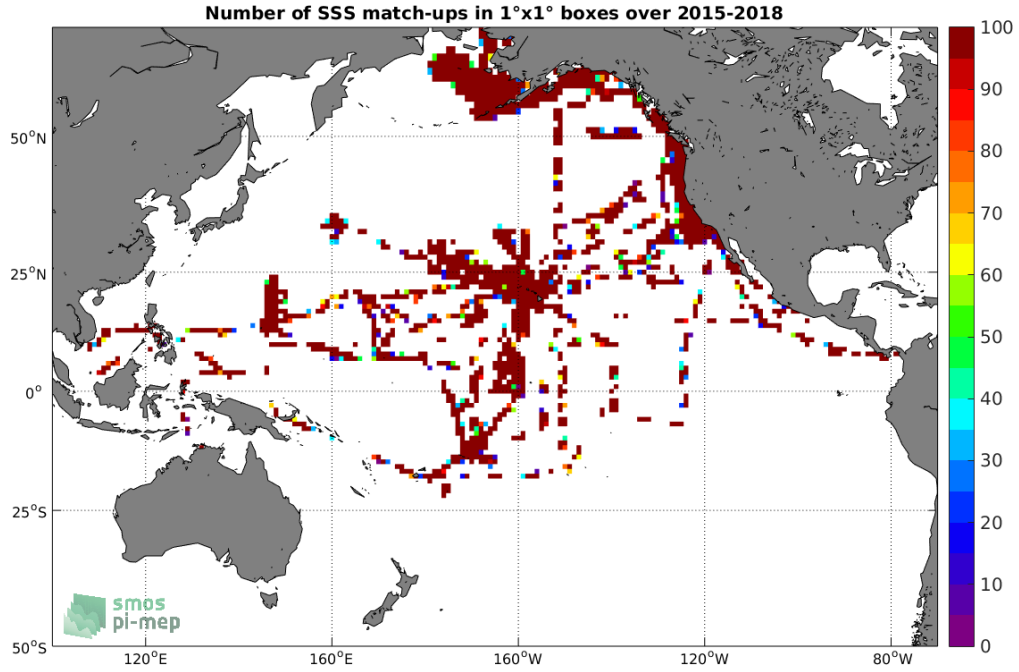
Figure 4: Number of SSS match-ups between TSG-SAMOS SSS and the SMAP-L2-JPL-V4 SSS product for the Pacific Ocean Pi-MEP region over 1^\circ \times 1^\circ boxes and for the full satellite product period.
