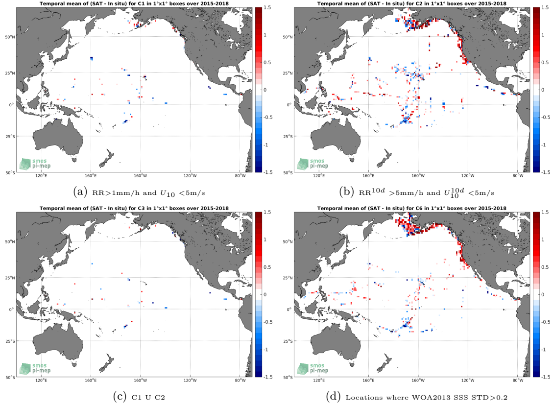
Figure 12: Temporal mean gridded over spatial boxes of size 1^\circ \times 1^\circ of \Delta SSS (SMAP-L2-JPL-V4 - TSG-SAMOS) for 4 different subdatasets corresponding to: RR > 1mm/h and U_{10} < 5\text{m/s} (a), RR^{10d} > 5\text{mm/h} and U_{10}^{10d} < 5\text{m/s} (b), C1 U C2 (c), Locations where WOA2013 SSS STD > 0.2 (d).
