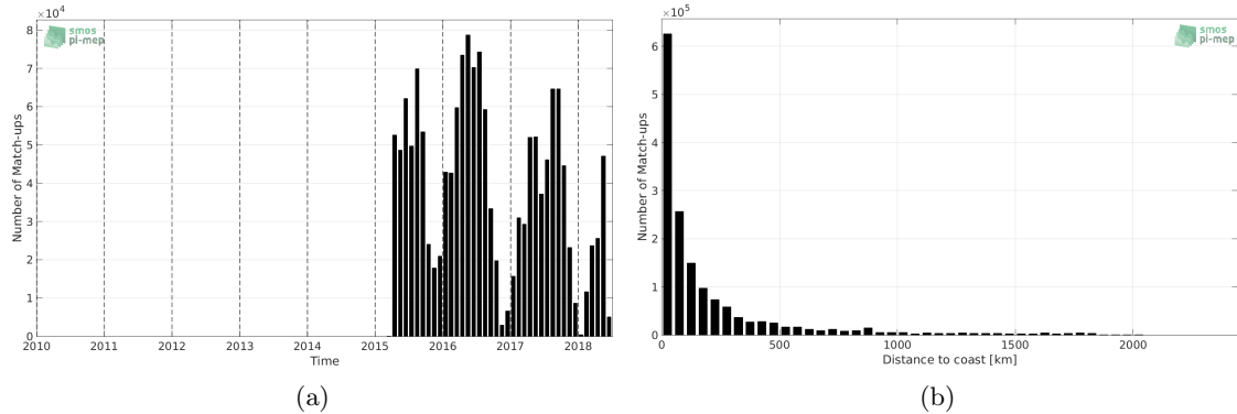
Figure 1: Number of match-ups between TSG-SAMOS and SMAP-L2-JPL-V4 SSS as a function of time (a) and as function of the distance to coast (b) over the Pacific Ocean Pi-MEP region and for the full satellite product period.
