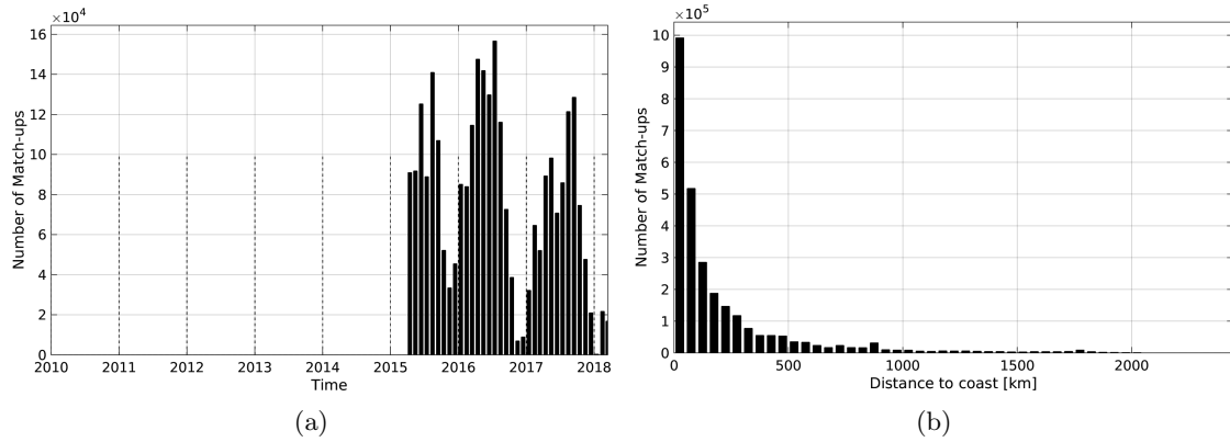
Figure 1: Number of match-ups between TSG-SAMOS and SMAP-L2-JPL-V4 SSS as a function of time (a) and as function of the distance to coast (b) over the Pacific Ocean Pi-MEP region and for the full satellite product period.
