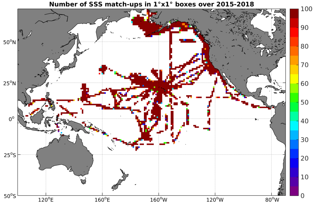
Figure 4: Number of SSS match-ups between TSG-SAMOS SSS and the SMAP-L2-JPL-V4 SSS product for the Pacific Ocean Pi-MEP region over 1^\circ \times 1^\circ boxes and for the full satellite product period.
