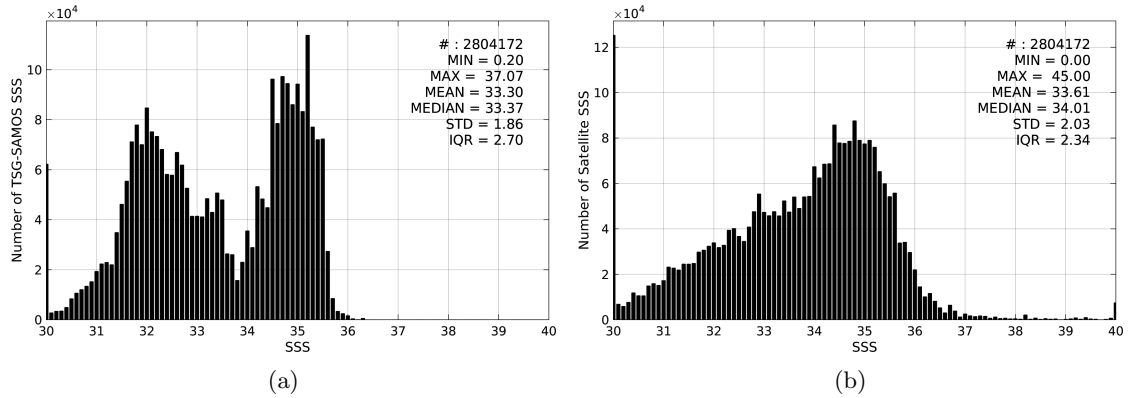
Figure 2: Histograms of SSS from TSG-SAMOS (a) and SMAP-L2-JPL-V4 (b) considering all match-up pairs per bins of 0.1 over the Pacific Ocean Pi-MEP region and for the full satellite product period.
