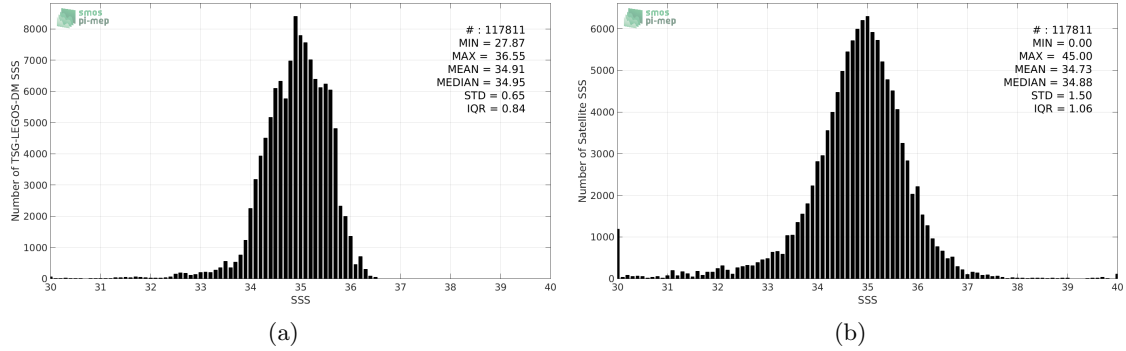
Figure 2: Histograms of SSS from TSG-LEGOS-DM (a) and SMAP-L2-JPL-V4 (b) considering all match-up pairs per bins of 0.1 over the Pacific Ocean Pi-MEP region and for the full satellite product period.
