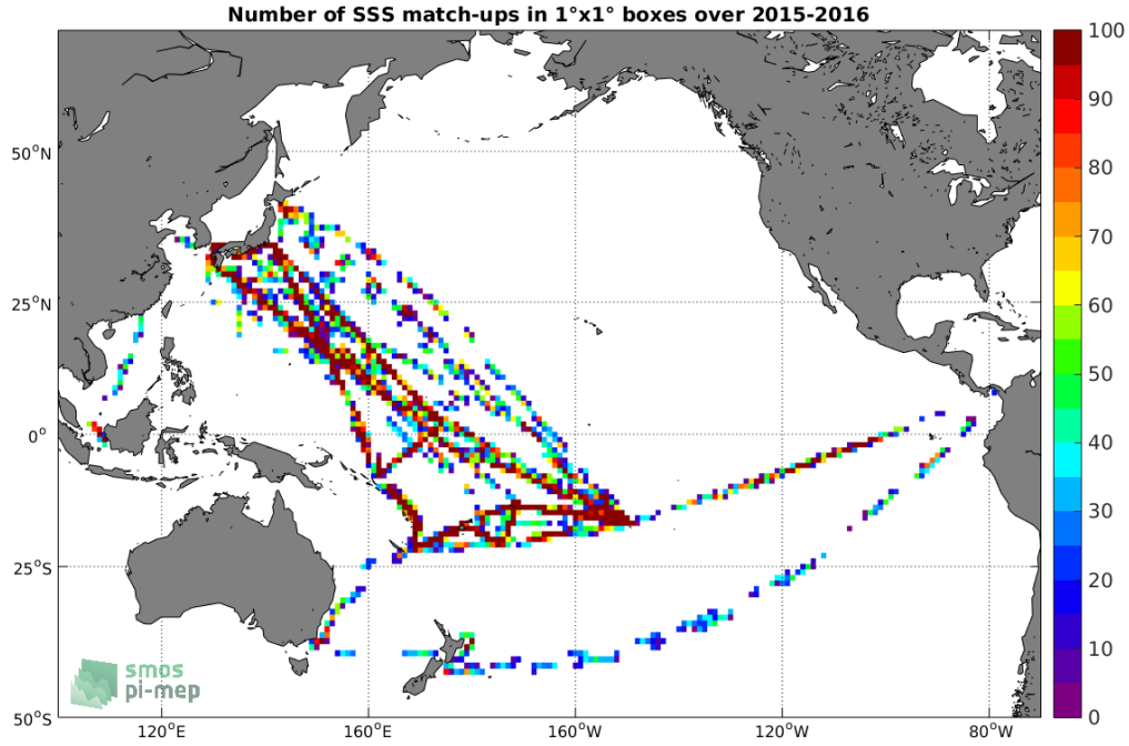
Figure 4: Number of SSS match-ups between TSG-LEGOS-DM SSS and the SMAP-L2-JPL-V4 SSS product for the Pacific Ocean Pi-MEP region over 1^\circ \times 1^\circ boxes and for the full satellite product period.
