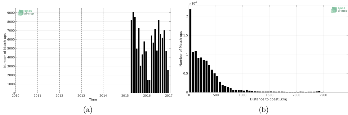
Figure 1: Number of match-ups between TSG-LEGOS-DM and SMAP-L2-JPL-V4 SSS as a function of time (a) and as function of the distance to coast (b) over the Pacific Ocean Pi-MEP region and for the full satellite product period.
