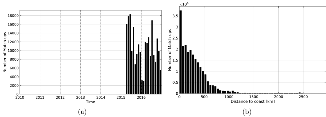
Figure 1: Number of match-ups between TSG-LEGOS-DM and SMAP-L2-JPL-V4 SSS as a function of time (a) and as function of the distance to coast (b) over the Pacific Ocean Pi-MEP region and for the full satellite product period.
