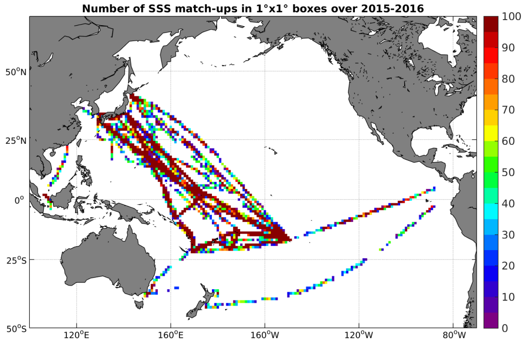
Figure 4: Number of SSS match-ups between TSG-LEGOS-DM SSS and the SMAP-L2-JPL-V4 SSS product for the Pacific Ocean Pi-MEP region over 1^\circ \times 1^\circ boxes and for the full satellite product period.
