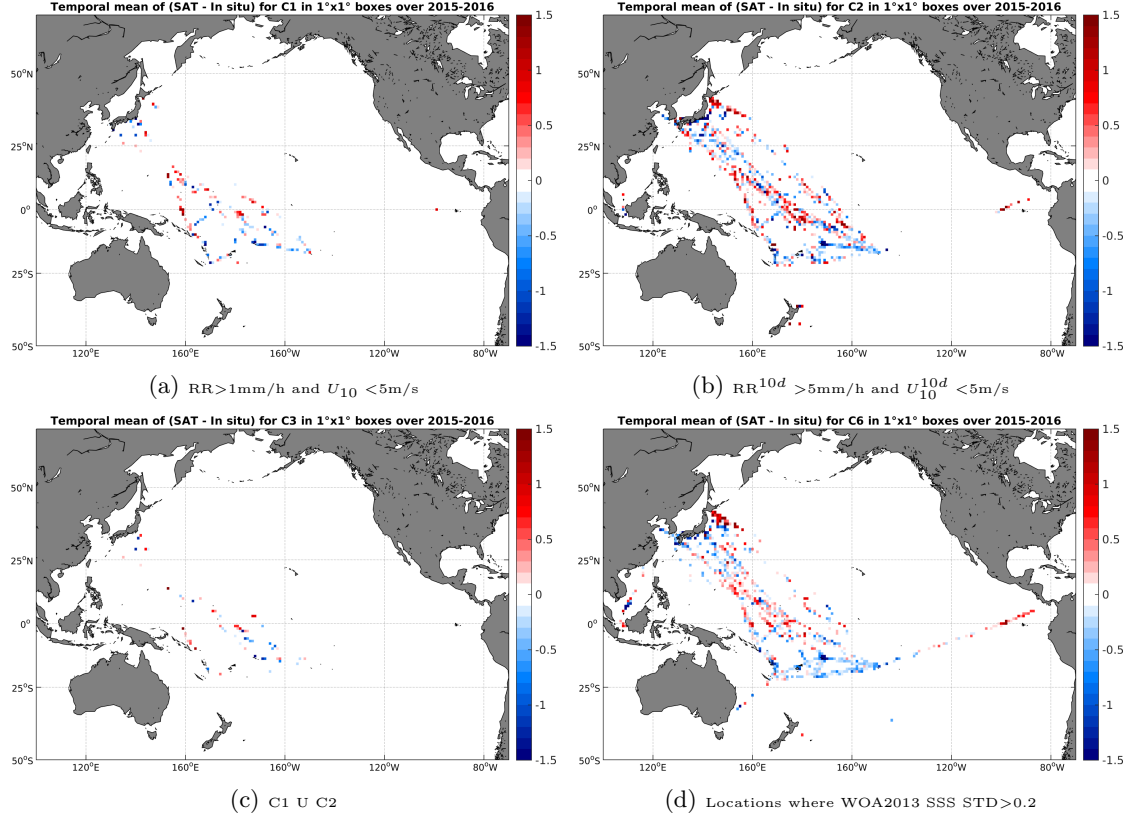
Figure 12: Temporal mean gridded over spatial boxes of size 1^\circ \times 1^\circ of \Delta SSS (SMAP-L2-JPL-V4 - TSG-LEGOS-DM) for 4 different subdatasets corresponding to: RR > 1 mm/h and U_{10} < 5 m/s (a), RR 10d > 5 mm/h and U_{10}^{10d} < 5 m/s (b), C1 U C2 (c), Locations where WOA2013 SSS STD > 0.2 (d).
