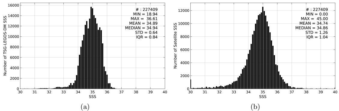
Figure 2: Histograms of SSS from TSG-LEGOS-DM (a) and SMAP-L2-JPL-V4 (b) considering all match-up pairs per bins of 0.1 over the Pacific Ocean Pi-MEP region and for the full satellite product period.
