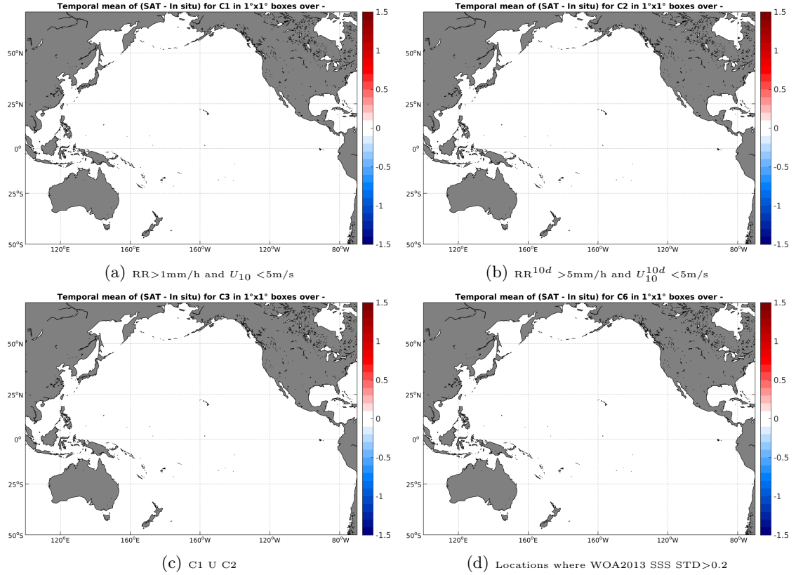
Figure 12: Temporal mean gridded over spatial boxes of size 1^\circ \times 1^\circ of \Delta SSS (SMAP-L2-JPL-V4 - TSG-GOSUD-Sailing-ship) for 4 different subdatasets corresponding to: RR > 1\text{mm/h} and U_{10} < 5\text{m/s} (a), RR^{10d} > 5\text{mm/h} and U_{10}^{10d} < 5\text{m/s} (b), C1 \cup C2 (c), Locations where WOA2013 SSS STD > 0.2 (d).
