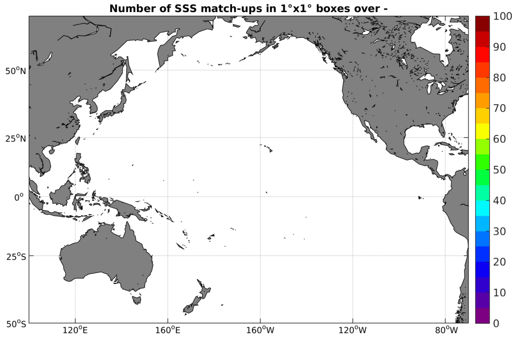
Figure 4: Number of SSS match-ups between TSG-GOSUD-Sailing-ship SSS and the SMAP-L2-JPL-V4 SSS product for the Pacific Ocean Pi-MEP region over 1^\circ \times 1^\circ boxes and for the full satellite product period.
