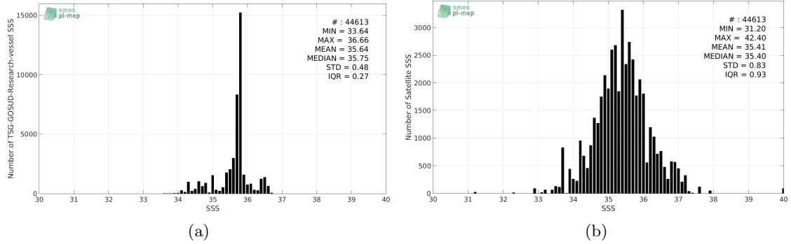
Figure 2: Histograms of SSS from TSG-GOSUD-Research-vessel (a) and SMAP-L2-JPL-V4 (b) considering all match-up pairs per bins of 0.1 over the Pacific Ocean Pi-MEP region and for the full satellite product period.
