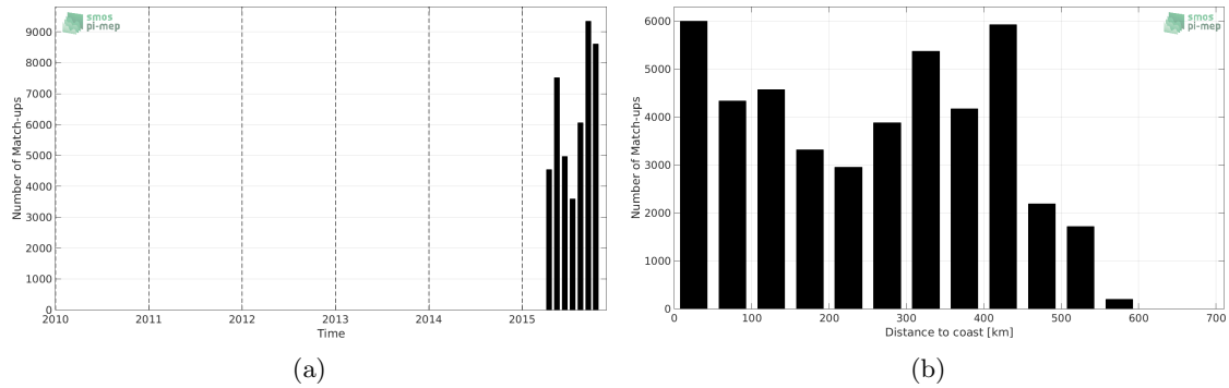
Figure 1: Number of match-ups between TSG-GOSUD-Research-vessel and SMAP-L2-JPL-V4 SSS as a function of time (a) and as function of the distance to coast (b) over the Pacific Ocean Pi-MEP region and for the full satellite product period.
