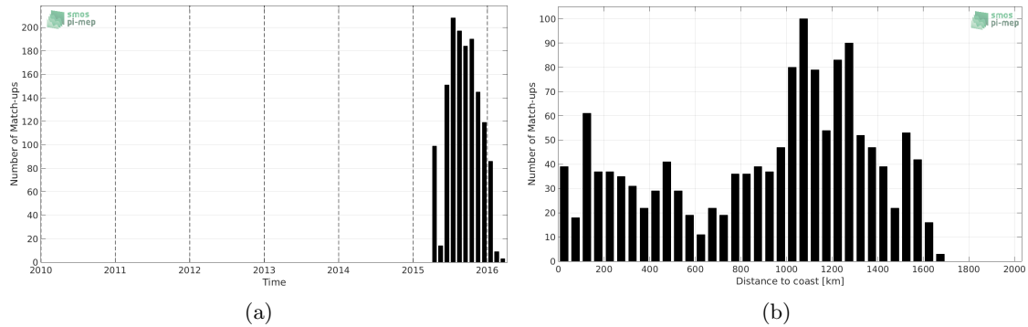
Figure 1: Number of match-ups between Sea mammals and SMAP-L2-JPL-V4 SSS as a function of time (a) and as function of the distance to coast (b) over the Pacific Ocean Pi-MEP region and for the full satellite product period.
