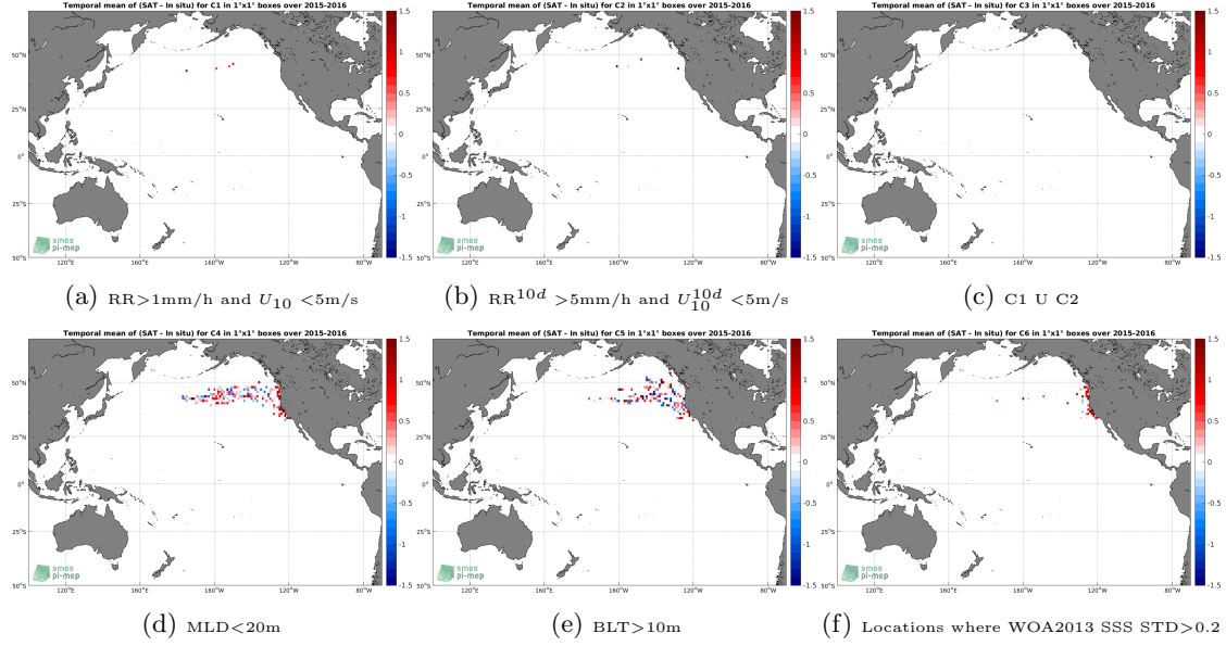
Figure 12: Temporal mean gridded over spatial boxes of size 1^\circ \times 1^\circ of \Delta\text{SSS} (SMAP-L2-JPL-V4 - Sea mammals) for 6 different subdatasets corresponding to: \text{RR} > 1\text{mm/h} and U_{10} < 5\text{m/s} (a), \text{RR}^{10d} > 5\text{mm/h} and U_{10}^{10d} < 5\text{m/s} (b), C1 U C2 (c), \text{MLD} < 20\text{m} (d), \text{BLT} > 10\text{m} (e), Locations where WOA2013 SSS STD > 0.2 (f).
