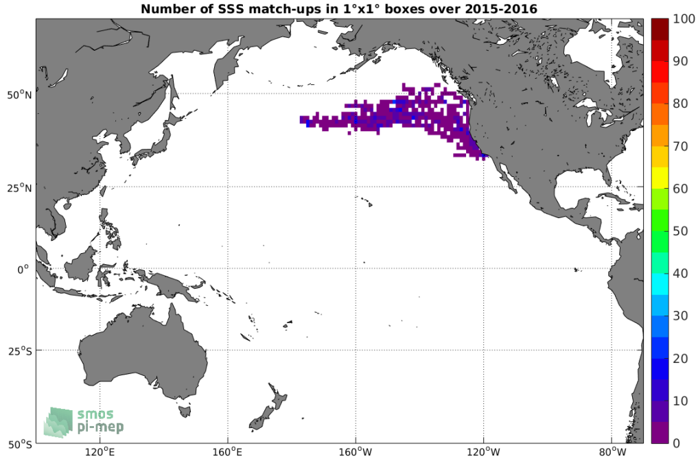
Figure 4: Number of SSS match-ups between Sea mammals SSS and the SMAP-L2-JPL-V4 SSS product for the Pacific Ocean Pi-MEP region over 1^\circ \times 1^\circ boxes and for the full satellite product period.
