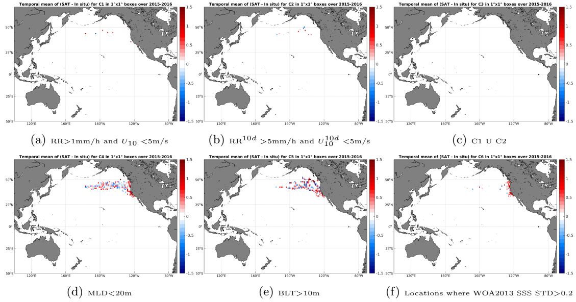
Figure 12: Temporal mean gridded over spatial boxes of size 1^\circ \times 1^\circ of \Delta SSS (SMAP-L2-JPL-V4 - Sea mammals) for 6 different subdatasets corresponding to: RR > 1mm/h and U_{10} < 5 m/s (a), RR^{10d} > 5 mm/h and U_{10}^{10d} < 5 m/s (b), C1 U C2 (c), MLD < 20m (d), BLT > 10m (e), Locations where WOA2013 SSS STD > 0.2 (f).
