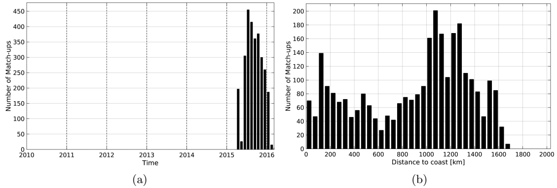
Figure 1: Number of match-ups between Sea mammals and SMAP-L2-JPL-V4 SSS as a function of time (a) and as function of the distance to coast (b) over the Pacific Ocean Pi-MEP region and for the full satellite product period.
