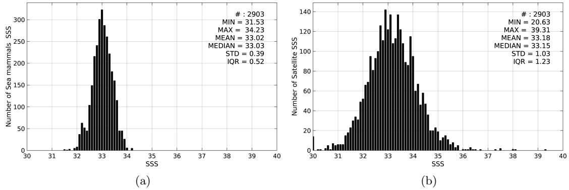
Figure 2: Histograms of SSS from Sea mammals (a) and SMAP-L2-JPL-V4 (b) considering all match-up pairs per bins of 0.1 over the Pacific Ocean Pi-MEP region and for the full satellite product period.
