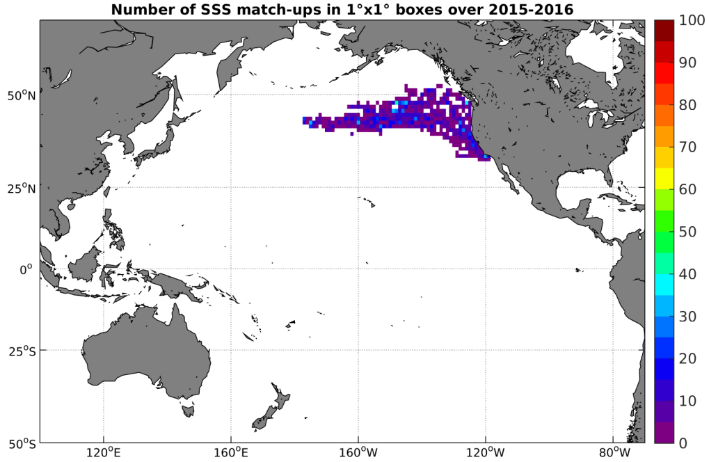
Figure 4: Number of SSS match-ups between Sea mammals SSS and the SMAP-L2-JPL-V4 SSS product for the Pacific Ocean Pi-MEP region over 1^\circ \times 1^\circ boxes and for the full satellite product period.
