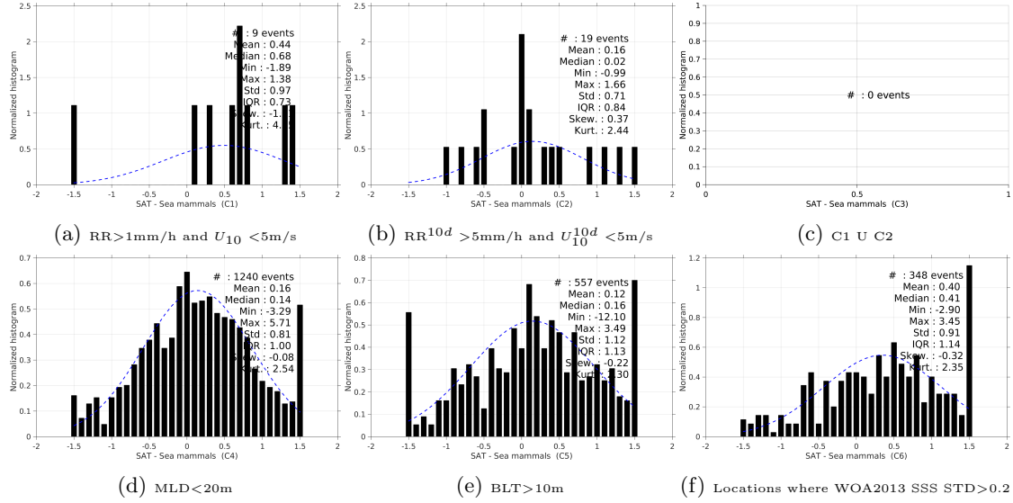
Figure 13: Normalized histogram of \Delta SSS (SMAP-L2-JPL-V4 - Sea mammals) for 6 different sub-datasets corresponding to: RR > 1\text{mm/h} and U_{10} < 5\text{m/s} (a), RR^{10d} > 5\text{mm/h} and U_{10}^{10d} < 5\text{m/s} (b), C1 U C2 (c), MLD < 20\text{m} (d), BLT > 10\text{m} (e), Locations where WOA2013 SSS STD > 0.2 (f).
