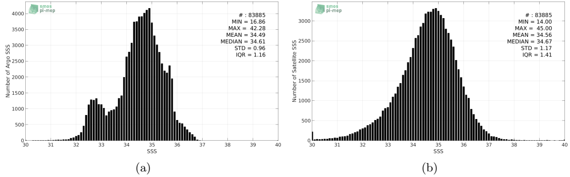
Figure 2: Histograms of SSS from Argo (a) and SMAP-L2-JPL-V4 (b) considering all match-up pairs per bins of 0.1 over the Pacific Ocean Pi-MEP region and for the full satellite product period.
