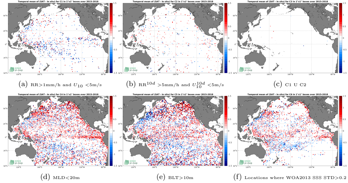
Figure 12: Temporal mean gridded over spatial boxes of size 1^\circ \times 1^\circ of \Delta\text{SSS} (SMAP-L2-JPL-V4 - Argo) for 6 different subdatasets corresponding to: \text{RR} > 1\text{mm/h} and U_{10} < 5\text{m/s} (a), \text{RR}^{10d} > 5\text{mm/h} and U_{10}^{10d} < 5\text{m/s} (b), C1 U C2 (c), \text{MLD} < 20\text{m} (d), \text{BLT} > 10\text{m} (e), Locations where WOA2013 SSS STD > 0.2 (f).
