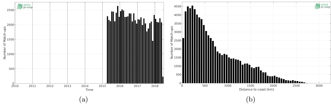
Figure 1: Number of match-ups between Argo and SMAP-L2-JPL-V4 SSS as a function of time (a) and as function of the distance to coast (b) over the Pacific Ocean Pi-MEP region and for the full satellite product period.
