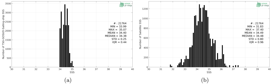
Figure 2: Histograms of SSS from TSG-GOSUD-Sailing-ship (a) and SMAP-L2-JPL-V4.3 (b) considering all match-up pairs per bins of 0.1 over the Pacific Ocean Pi-MEP region and for the full satellite product period.
