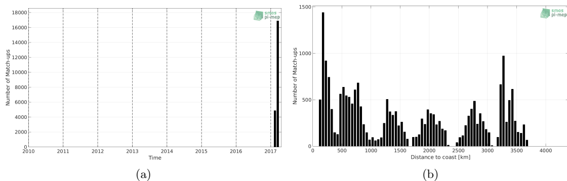
Figure 1: Number of match-ups between TSG-GOSUD-Sailing-ship and SMAP-L2-JPL-V4.3 SSS as a function of time (a) and as function of the distance to coast (b) over the Pacific Ocean Pi-MEP region and for the full satellite product period.
