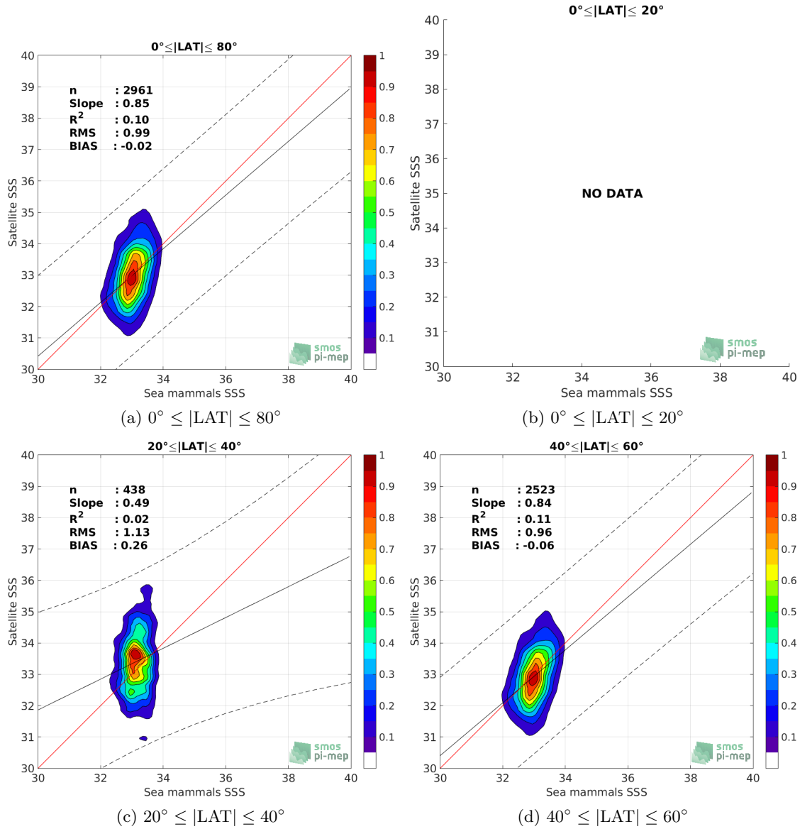
Figure 9: Contour maps of the concentration of SMAP-L2-JPL-V4.3 SSS (y-axis) versus Sea mammals SSS (x-axis) at match-up pairs for different latitude bands. For each plot, the red line shows x=y . The black thin and dashed lines indicate a linear fit through the data cloud and the \pm 95\% confidence levels, respectively. The number match-up pairs n , the slope and R^2 coefficient of the linear fit, the root mean square (RMS) and the mean bias between satellite and in situ data are indicated for each latitude band in each plots.
