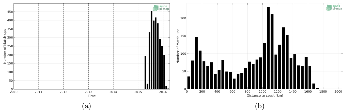
Figure 1: Number of match-ups between Sea mammals and SMAP-L2-JPL-V4.3 SSS as a function of time (a) and as function of the distance to coast (b) over the Pacific Ocean Pi-MEP region and for the full satellite product period.
