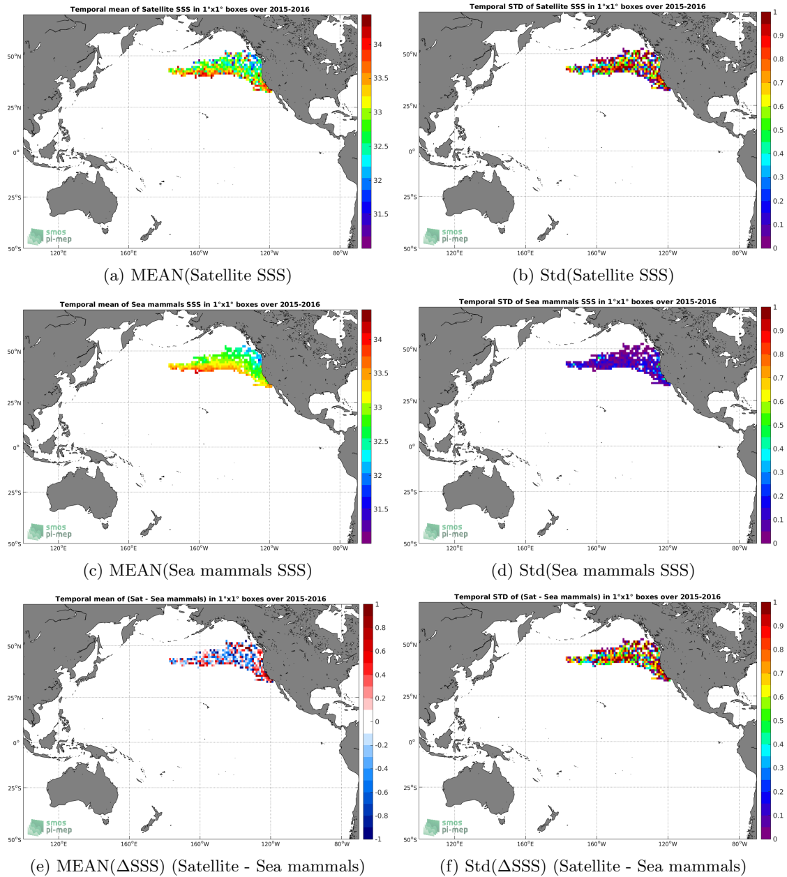
Figure 6: Temporal mean (left) and Std (right) of SSS from SMAP-L2-JPL-V4.3 (top), Sea mammals (middle), and of \Delta SSS (Satellite - Sea mammals). Only match-up pairs are used to generate these maps.
