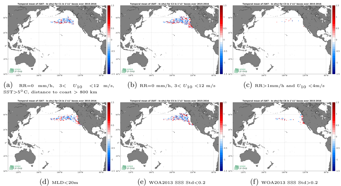
Figure 12: Temporal mean gridded over spatial boxes of size 1^\circ \times 1^\circ of \Delta SSS (SMAP-L2-JPL-V4.3 - Sea mammals) for 6 different subdatasets corresponding to:RR=0 mm/h, 3 < U_{10} < 12 m/s, SST >5^\circ C, distance to coast > 800 km (a), RR=0 mm/h, 3 < U_{10} < 12 m/s (b), RR >1 mm/h and U_{10} < 4 m/s (c),MLD <20 m (d),WOA2013 SSS Std <0.2 (e),WOA2013 SSS Std >0.2 (f).
