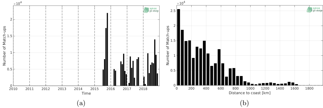
Figure 1: Number of match-ups between TSG-GOSUD-Research-vessel and SMAP-L2-JPL-V4.2 SSS as a function of time (a) and as function of the distance to coast (b) over the Pacific Ocean Pi-MEP region and for the full satellite product period.
