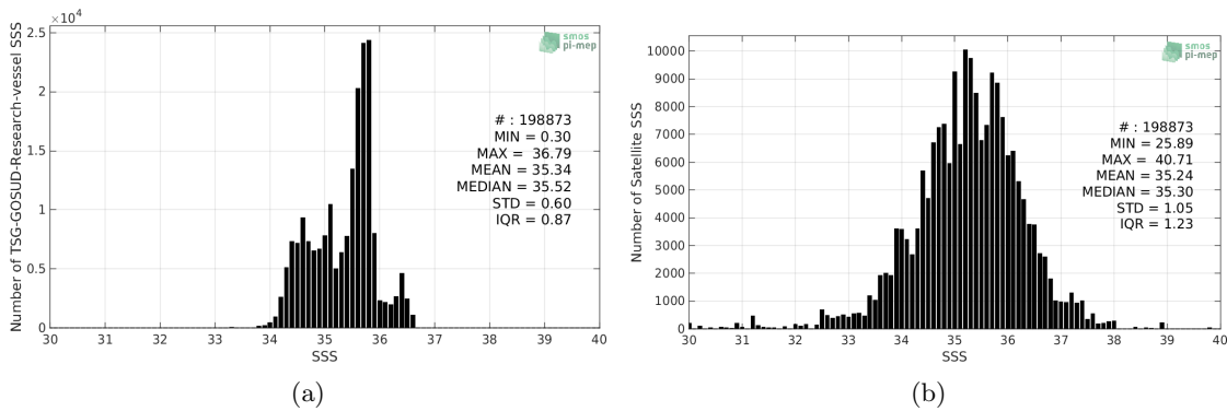
Figure 2: Histograms of SSS from TSG-GOSUD-Research-vessel (a) and SMAP-L2-JPL-V4.2 (b) considering all match-up pairs per bins of 0.1 over the Pacific Ocean Pi-MEP region and for the full satellite product period.
