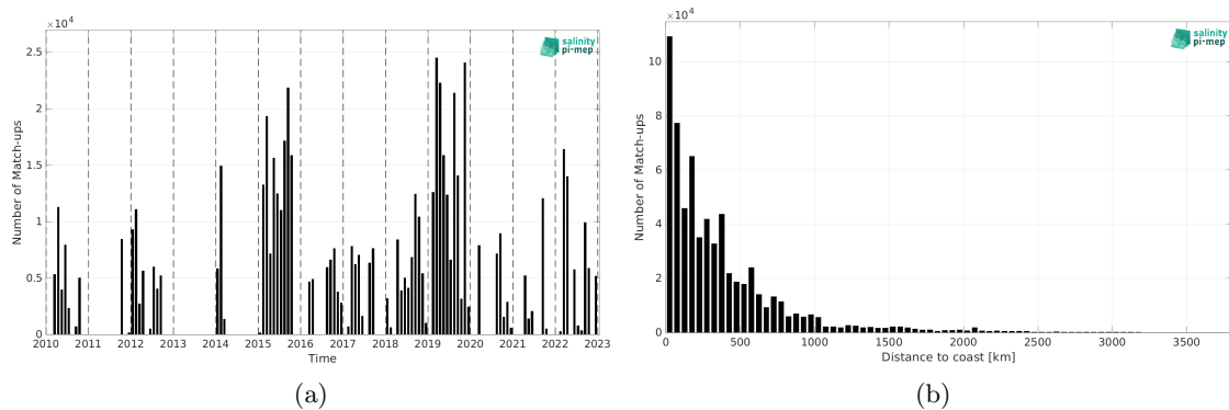
Figure 2: Number of match-ups between TSG (GOSUD-Research-vessel) and ISAS v7 - Monthly (Ifremer-LOPS-CMEMS) SSS as a function of time (a) and as function of the distance to coast (b) over the Pacific Ocean Pi-MEP region and for the full satellite product period.
