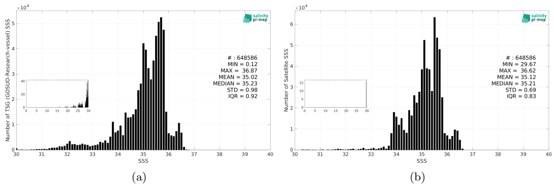
Figure 3: Histograms of SSS from TSG (GOSUD-Research-vessel) (a) and ISAS v7 - Monthly (Ifremer-LOPS-CMEMS) (b) considering all match-up pairs per bins of 0.1 over the Pacific Ocean Pi-MEP region and for the full satellite product period.
