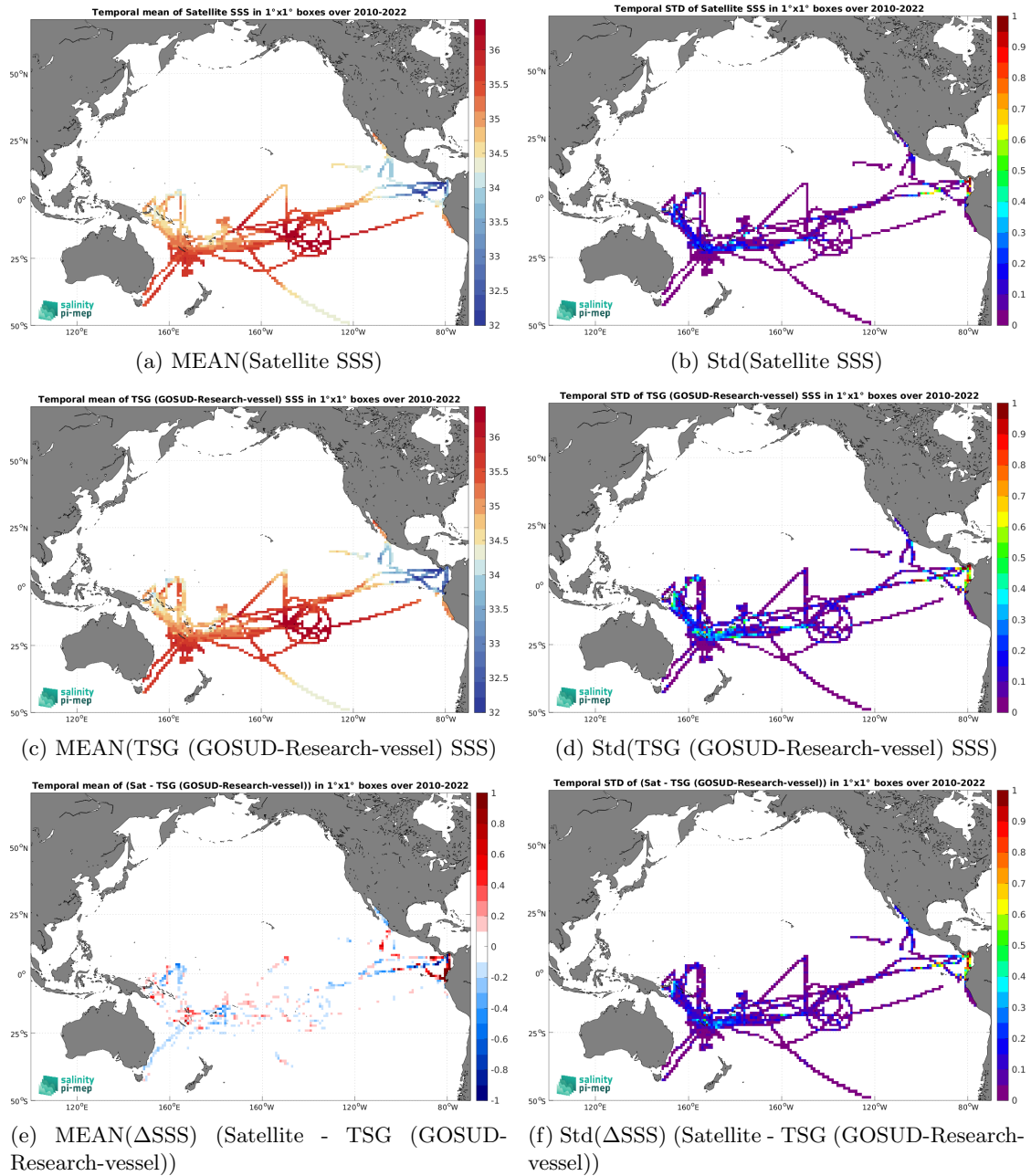
Figure 7: Temporal mean (left) and Std (right) of SSS from ISAS v7 - Monthly (Ifremer-LOPS-CMEMS) (top), TSG (GOSUD-Research-vessel) (middle), and of \Delta SSS (Satellite - TSG (GOSUD-Research-vessel)). Only match-up pairs are used to generate these maps.
