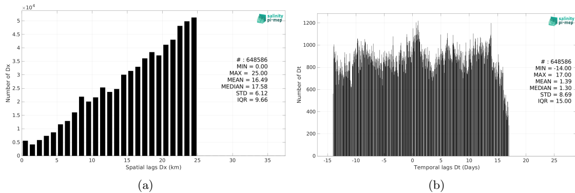
Figure 6: Histograms of the spatial (a) and temporal (b) lags between the location/time of the TSG (GOSUD-Research-vessel) measurement and the date of the corresponding ISAS v7 - Monthly (Ifremer-LOPS-CMEMS) SSS pixel.
