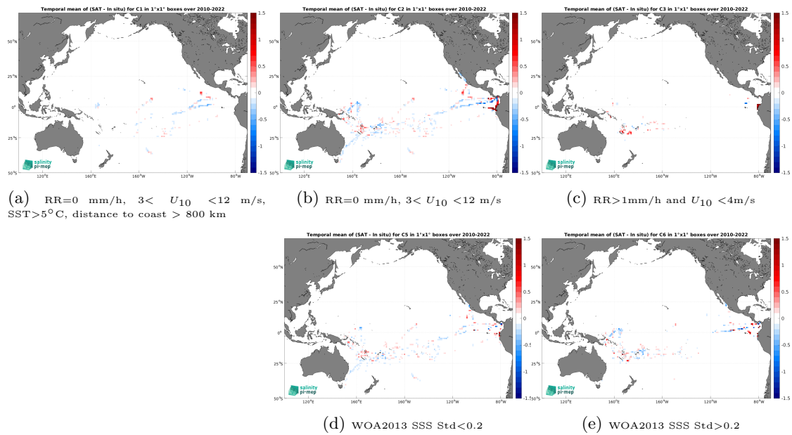
Figure 14: Temporal mean gridded over spatial boxes of size 1^\circ \times 1^\circ of \Delta SSS (ISAS v7 - Monthly (Ifremer-LOPS-CMEMS) - TSG (GOSUD-Research-vessel)) for 5 different subdatasets corresponding to:RR=0 mm/h, 3 < U_{10} < 12 m/s, SST >5^\circ\text{C} , distance to coast > 800 km (a), RR=0 mm/h, 3 < U_{10} < 12 m/s (b), RR >1 mm/h and U_{10} < 4 m/s (c), WOA2013 SSS Std <0.2 (d), WOA2013 SSS Std >0.2 (e).
