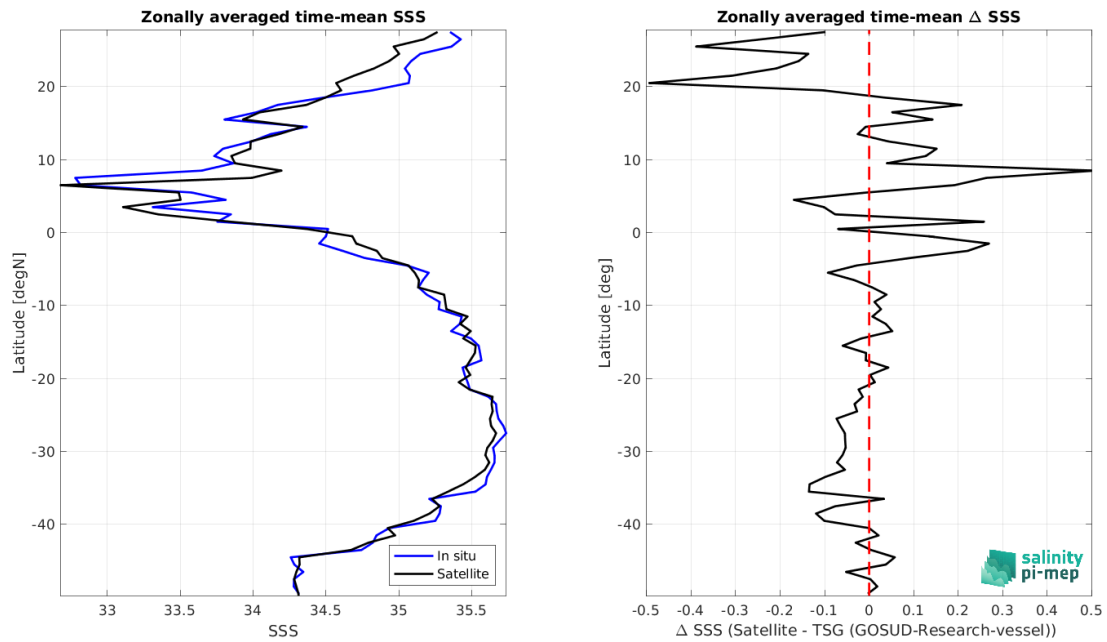
Figure 9: Left panel: Zonal mean SSS from ISAS v7 - Monthly (Ifremer-LOPS-CMEMS) satellite product (black) and from TSG (GOSUD-Research-vessel) (blue). Right panel: Zonal mean of \Delta SSS (Satellite - TSG (GOSUD-Research-vessel)) for all the collected Pi-MEP match-up pairs estimated over the full satellite product period.
