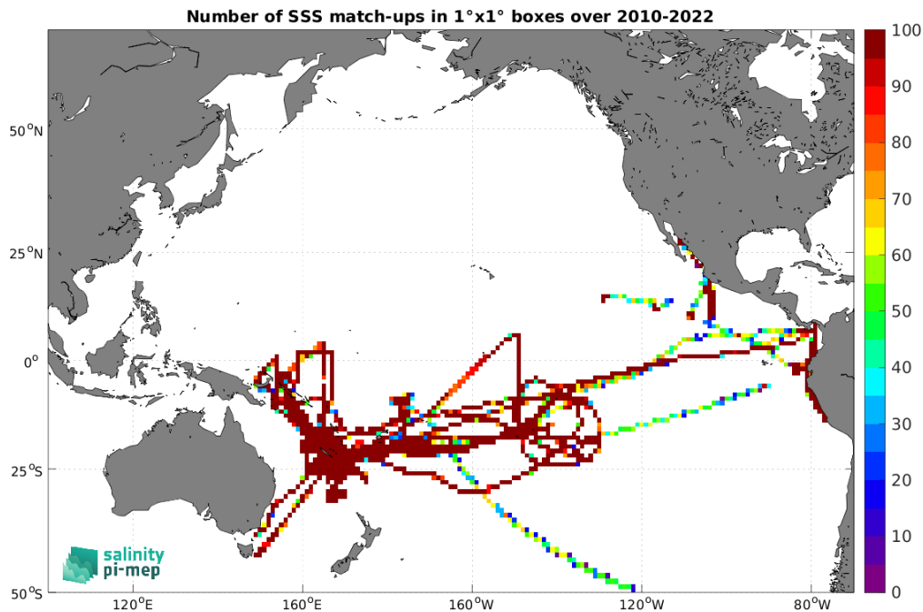
Figure 5: Number of SSS match-ups between TSG (GOSUD-Research-vessel) SSS and the ISAS v7 - Monthly (Ifremer-LOPS-CMEMS) SSS product for the Pacific Ocean Pi-MEP region over 1^\circ \times 1^\circ boxes and for the full satellite product period.
