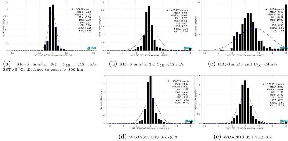
Figure 15: Normalized histogram of \Delta SSS (ISAS v7 - Monthly (Ifremer-LOPS-CMEMS) - TSG (GOSUD-Research-vessel)) for 5 different subdatasets corresponding to: RR=0 mm/h, 3 < U_{10} < 12 m/s, SST > 5°C, distance to coast > 800 km (a), RR=0 mm/h, 3 < U_{10} < 12 m/s (b), RR > 1mm/h and U_{10} < 4 m/s (c), WOA2013 SSS Std < 0.2 (d), WOA2013 SSS Std > 0.2 (e).
