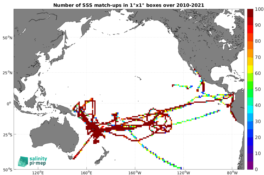
Figure 5: Number of SSS match-ups between TSG (GOSUD-Research-vessel) SSS and the ISAS SSS product for the Pacific Ocean Pi-MEP region over 1^\circ \times 1^\circ boxes and for the full satellite product period.
