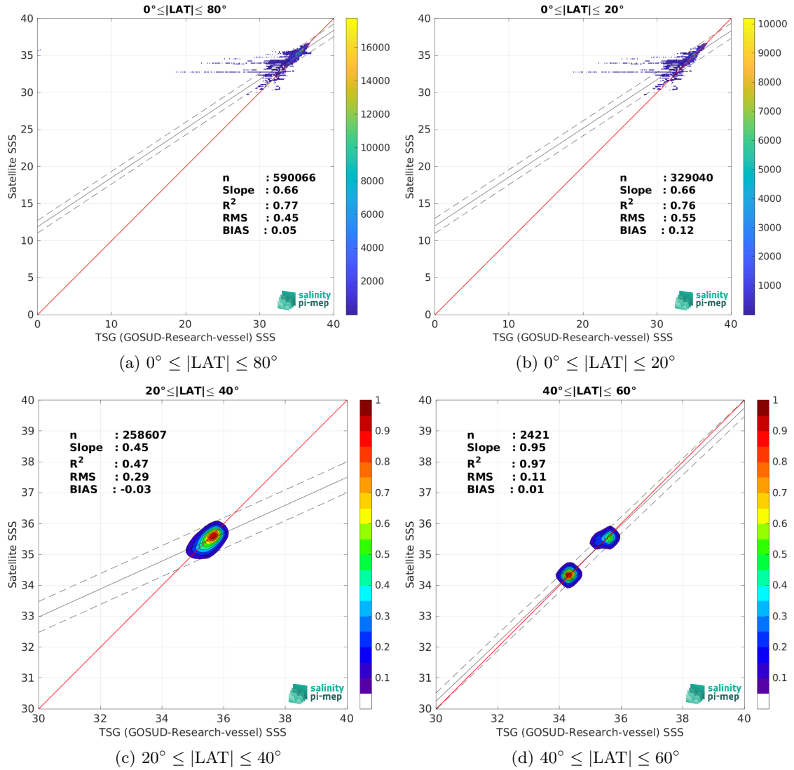
Figure 10: Contour maps of the concentration of ISAS SSS (y-axis) versus TSG (GOSUD-Research-vessel) SSS (x-axis) at match-up pairs for different latitude bands. For each plot, the red line shows x=y . The black thin and dashed lines indicate a linear fit through the data cloud and the \pm 95\% confidence levels, respectively. The number match-up pairs n , the slope and R^2 coefficient of the linear fit, the root mean square (RMS) and the mean bias between satellite and in situ data are indicated for each latitude band in each plots.
