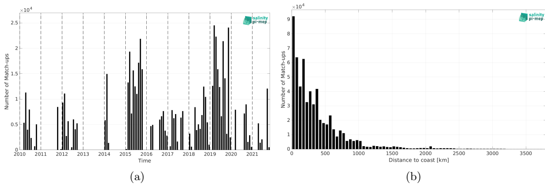
Figure 2: Number of match-ups between TSG (GOSUD-Research-vessel) and ISAS SSS as a function of time (a) and as function of the distance to coast (b) over the Pacific Ocean Pi-MEP region and for the full satellite product period.
