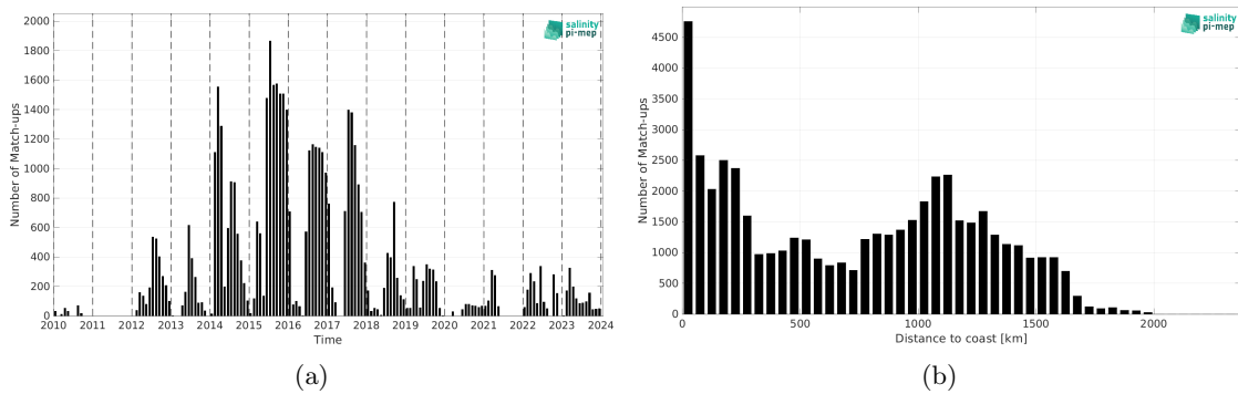
Figure 2: Number of match-ups between Marine mammals and ISAS v7 - Monthly (Ifremer-LOPS-CMEMS) SSS as a function of time (a) and as function of the distance to coast (b) over the Pacific Ocean Pi-MEP region and for the full satellite product period.
