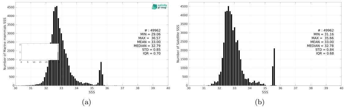
Figure 3: Histograms of SSS from Marine mammals (a) and ISAS v7 - Monthly (Ifremer-LOPS-CMEMS) (b) considering all match-up pairs per bins of 0.1 over the Pacific Ocean Pi-MEP region and for the full satellite product period.
