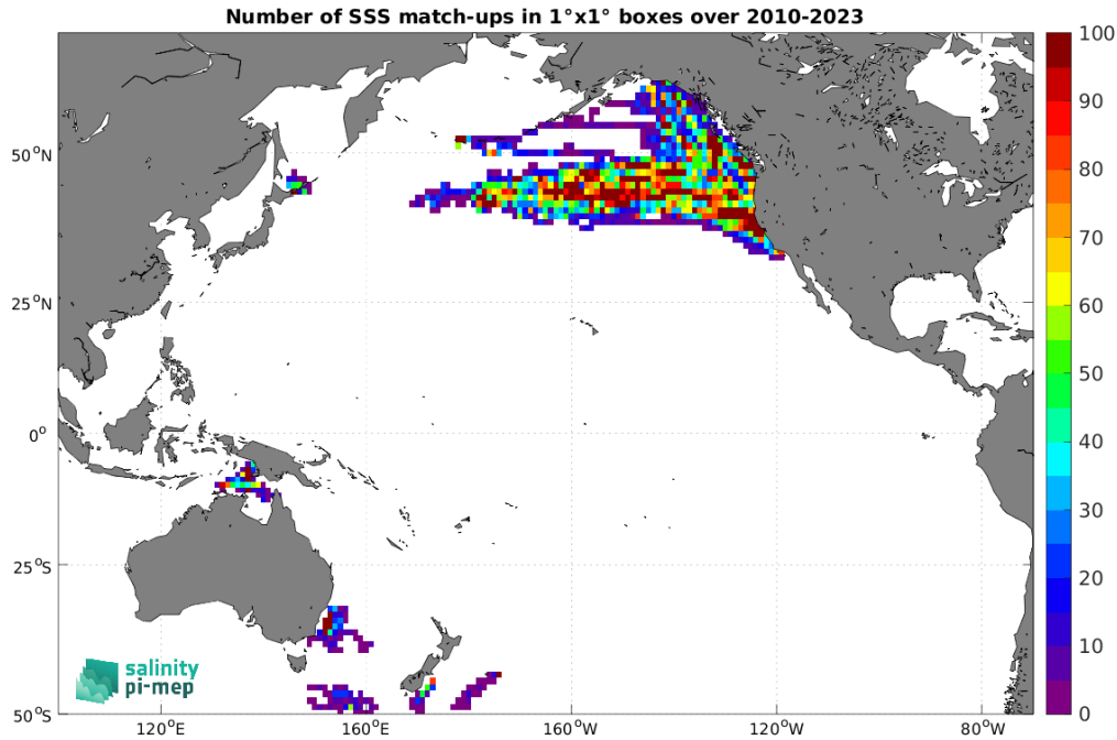
Figure 5: Number of SSS match-ups between Marine mammals SSS and the ISAS v7 - Monthly (Ifremer-LOPS-CMEMS) SSS product for the Pacific Ocean Pi-MEP region over 1^\circ \times 1^\circ boxes and for the full satellite product period.
