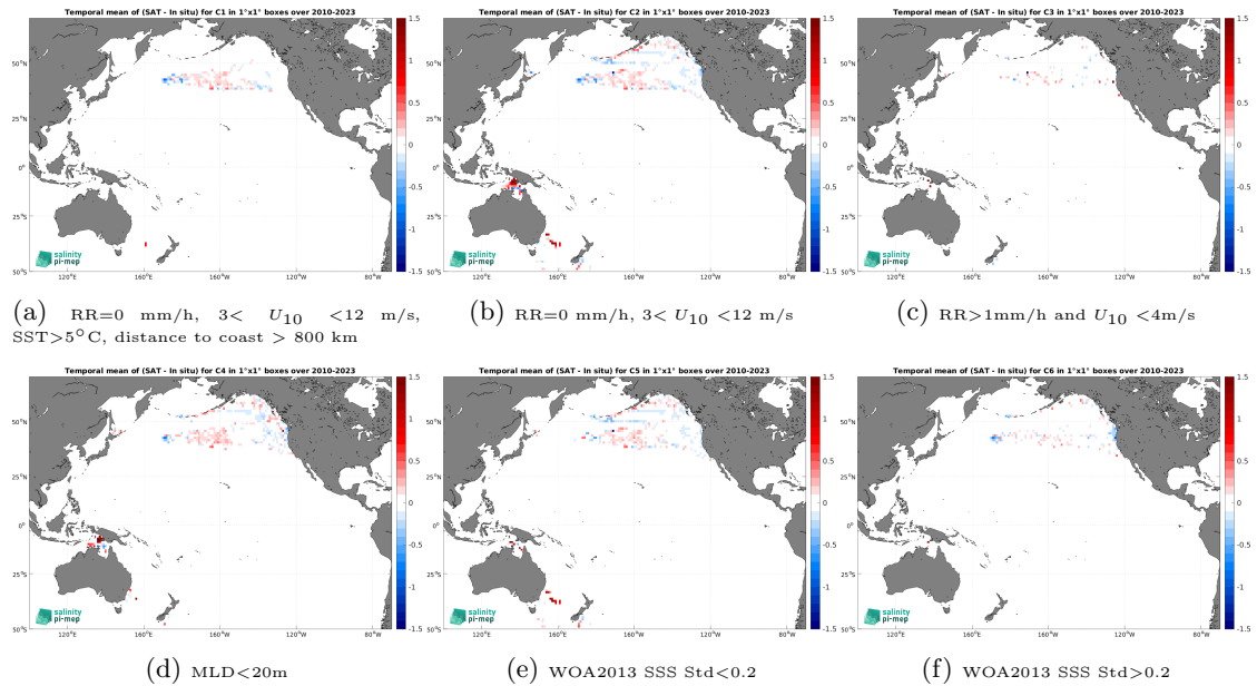
Figure 14: Temporal mean gridded over spatial boxes of size 1^\circ \times 1^\circ of \Delta SSS (ISAS v7 - Monthly (Ifremer-LOPS-CMEMS) - Marine mammals) for 6 different subdatasets corresponding to:RR=0 mm/h, 3 < U_{10} < 12 m/s, SST>5°C, distance to coast > 800 km (a), RR=0 mm/h, 3 < U_{10} < 12 m/s (b), RR>1mm/h and U_{10} < 4 m/s (c),MLD<20m (d),WOA2013 SSS Std<0.2 (e),WOA2013 SSS Std>0.2 (f).
