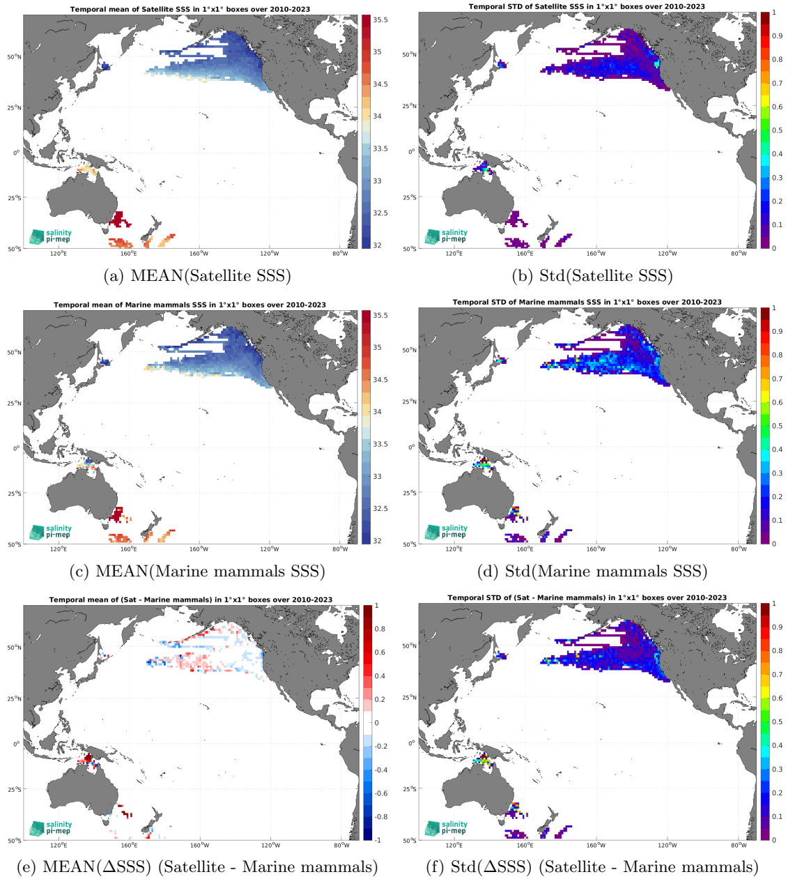
Figure 7: Temporal mean (left) and Std (right) of SSS from ISAS v7 - Monthly (Ifremer-LOPS-CMEMS) (top), Marine mammals (middle), and of \Delta SSS (Satellite - Marine mammals). Only match-up pairs are used to generate these maps.
