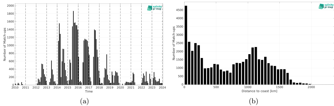
Figure 2: Number of match-ups between Marine mammals and ISAS SSS as a function of time (a) and as function of the distance to coast (b) over the Pacific Ocean Pi-MEP region and for the full satellite product period.
