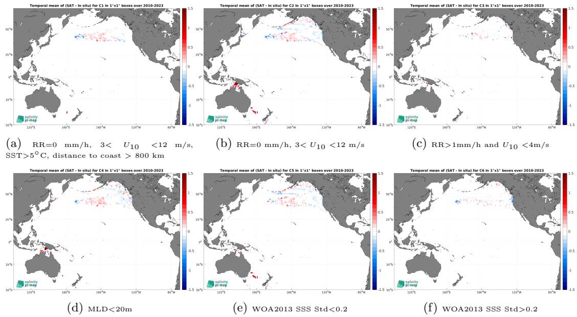
Figure 14: Temporal mean gridded over spatial boxes of size 1^\circ \times 1^\circ of \Delta SSS (ISAS - Marine mammals) for 6 different subdatasets corresponding to:RR=0 mm/h, 3 < U_{10} < 12 m/s, SST > 5^\circ\text{C} , distance to coast > 800 km (a), RR=0 mm/h, 3 < U_{10} < 12 m/s (b), RR > 1 mm/h and U_{10} < 4 m/s (c),MLD < 20 m (d),WOA2013 SSS Std < 0.2 (e),WOA2013 SSS Std > 0.2 (f).
