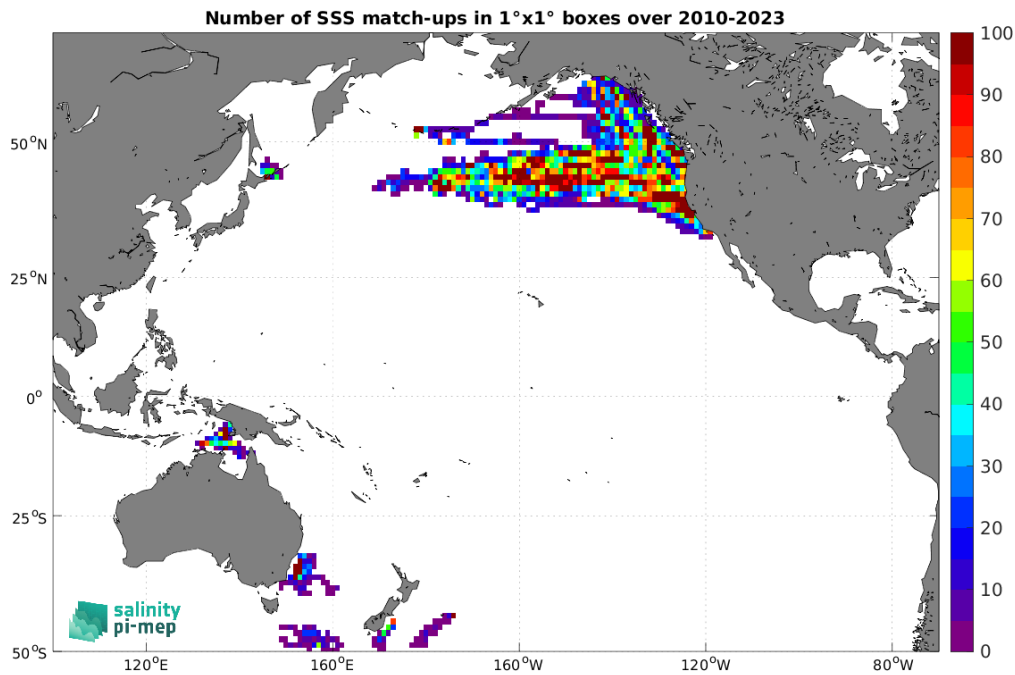
Figure 5: Number of SSS match-ups between Marine mammals SSS and the ISAS SSS product for the Pacific Ocean Pi-MEP region over 1^\circ \times 1^\circ boxes and for the full satellite product period.
