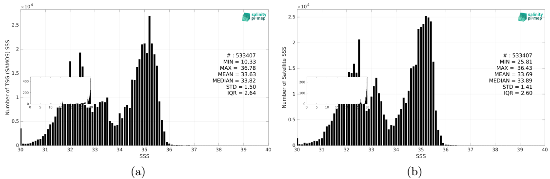
Figure 3: Histograms of SSS from TSG (SAMOS) (a) and CCI SSS L4 Merged-OI v5.5 - 7-day running (ESA) (b) considering all match-up pairs per bins of 0.1 over the Pacific Ocean Pi-MEP region and for the full satellite product period.
