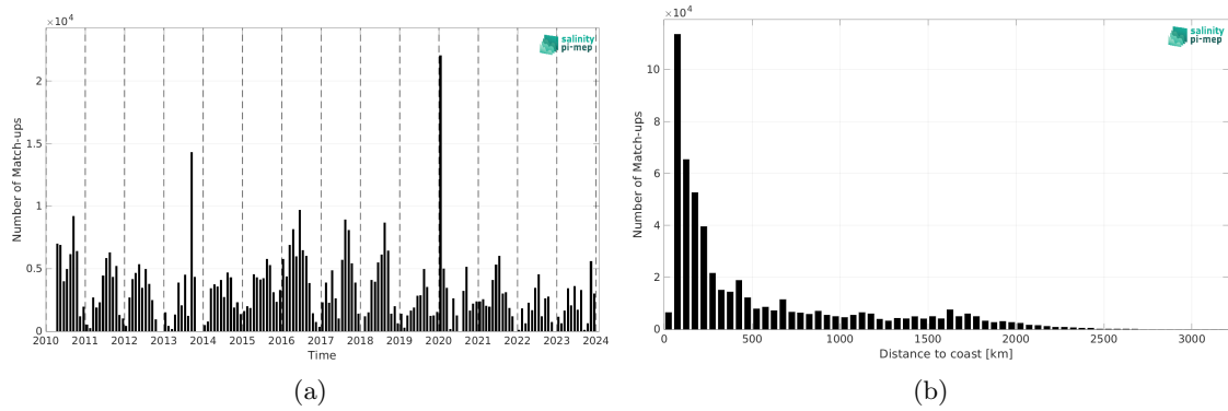
Figure 2: Number of match-ups between TSG (SAMOS) and CCI SSS L4 Merged-OI v5.5 - 7-day running (ESA) SSS as a function of time (a) and as function of the distance to coast (b) over the Pacific Ocean Pi-MEP region and for the full satellite product period.
