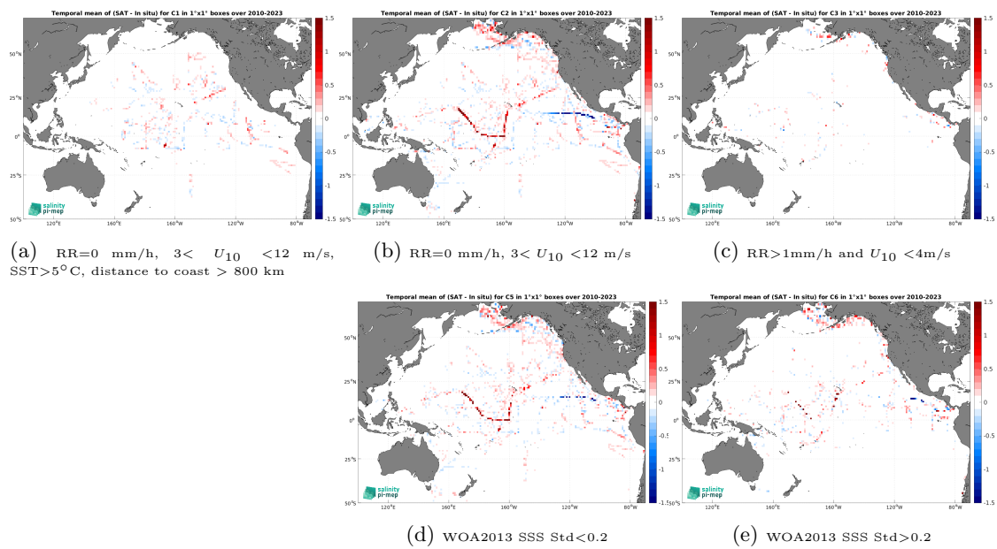
Figure 14: Temporal mean gridded over spatial boxes of size 1^\circ \times 1^\circ of \Delta SSS (CCI SSS L4 Merged-OI v5.5 - 7-day running (ESA) - TSG (SAMOS)) for 5 different subdatasets corresponding to: RR=0 mm/h, 3 < U_{10} < 12 m/s, SST > 5^\circ\text{C} , distance to coast > 800 km (a), RR=0 mm/h, 3 < U_{10} < 12 m/s (b), RR > 1 mm/h and U_{10} < 4 m/s (c), WOA2013 SSS Std < 0.2 (d), WOA2013 SSS Std > 0.2 (e).
