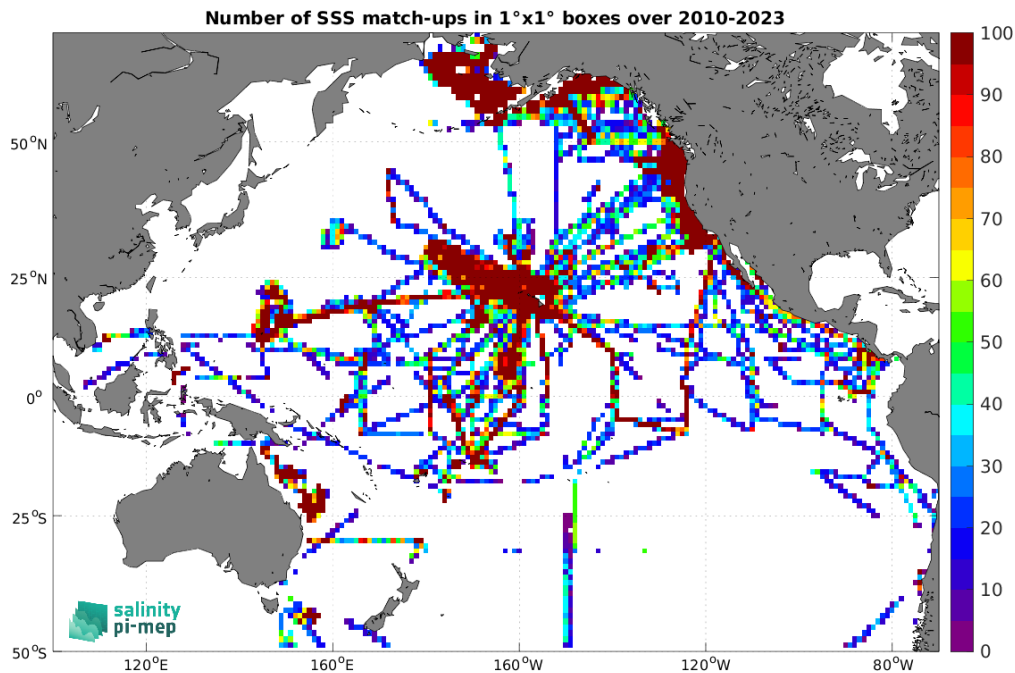
Figure 5: Number of SSS match-ups between TSG (SAMOS) SSS and the CCI SSS L4 Merged-OI v5.5 - 7-day running (ESA) SSS product for the Pacific Ocean Pi-MEP region over 1^\circ \times 1^\circ boxes and for the full satellite product period.
