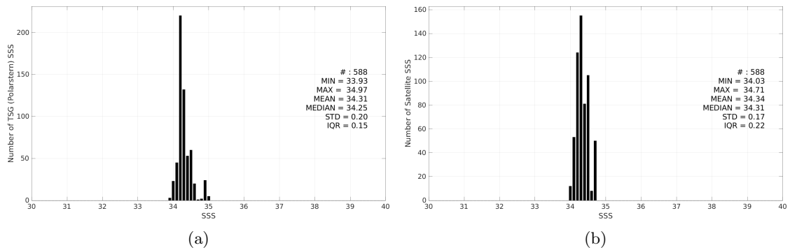
Figure 3: Histograms of SSS from TSG (Polarstern) (a) and CCI SSS L4 Merged-OI v5.5 - 7-day running (ESA) (b) considering all match-up pairs per bins of 0.1 over the Pacific Ocean Pi-MEP region and for the full satellite product period.
