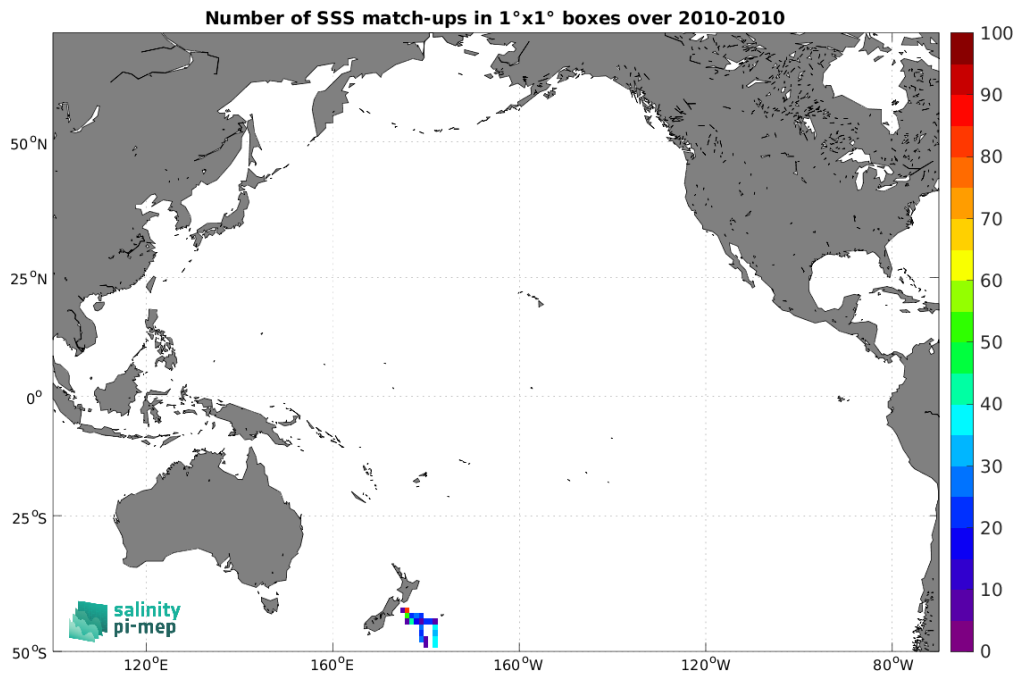
Figure 5: Number of SSS match-ups between TSG (Polarstern) SSS and the CCI SSS L4 Merged-OI v5.5 - 7-day running (ESA) SSS product for the Pacific Ocean Pi-MEP region over 1^\circ \times 1^\circ boxes and for the full satellite product period.
