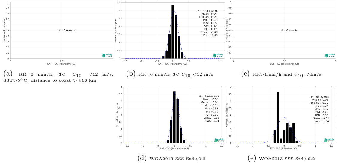
Figure 15: Normalized histogram of \Delta SSS (CCI SSS L4 Merged-OI v5.5 - 7-day running (ESA) - TSG (Polarstern)) for 5 different subdatasets corresponding to: RR=0 mm/h, 3 < U_{10} < 12 m/s, SST > 5°C, distance to coast > 800 km (a), RR=0 mm/h, 3 < U_{10} < 12 m/s (b), RR > 1mm/h and U_{10} < 4 m/s (c), WOA2013 SSS Std < 0.2 (d), WOA2013 SSS Std > 0.2 (e).
