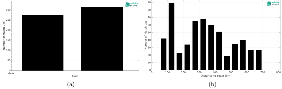
Figure 2: Number of match-ups between TSG (Polarstern) and CCI SSS L4 Merged-OI v5.5 - 7-day running (ESA) SSS as a function of time (a) and as function of the distance to coast (b) over the Pacific Ocean Pi-MEP region and for the full satellite product period.
