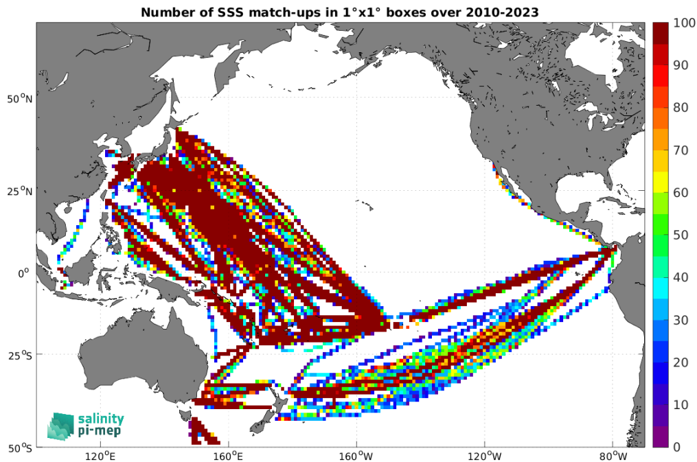
Figure 5: Number of SSS match-ups between TSG (LEGOS-DM) SSS and the CCI SSS L4 Merged-OI v5.5 - 7-day running (ESA) SSS product for the Pacific Ocean Pi-MEP region over 1^\circ \times 1^\circ boxes and for the full satellite product period.
