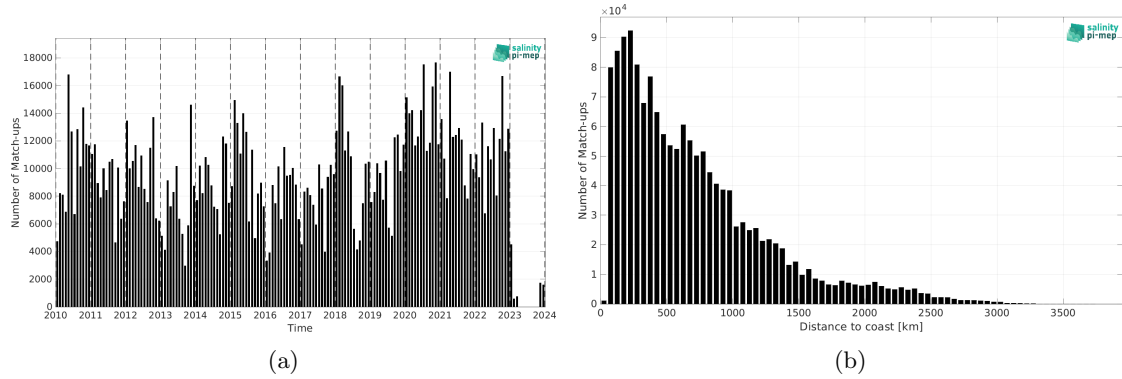
Figure 2: Number of match-ups between TSG (LEGOS-DM) and CCI SSS L4 Merged-OI v5.5 - 7-day running (ESA) SSS as a function of time (a) and as function of the distance to coast (b) over the Pacific Ocean Pi-MEP region and for the full satellite product period.
