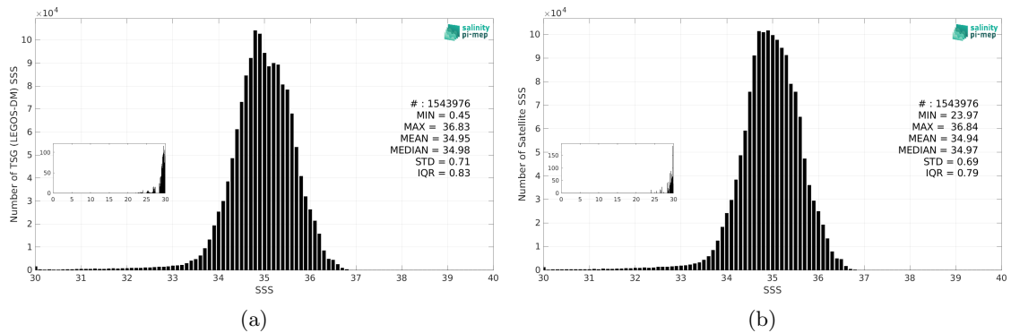
Figure 3: Histograms of SSS from TSG (LEGOS-DM) (a) and CCI SSS L4 Merged-OI v5.5 - 7-day running (ESA) (b) considering all match-up pairs per bins of 0.1 over the Pacific Ocean Pi-MEP region and for the full satellite product period.
