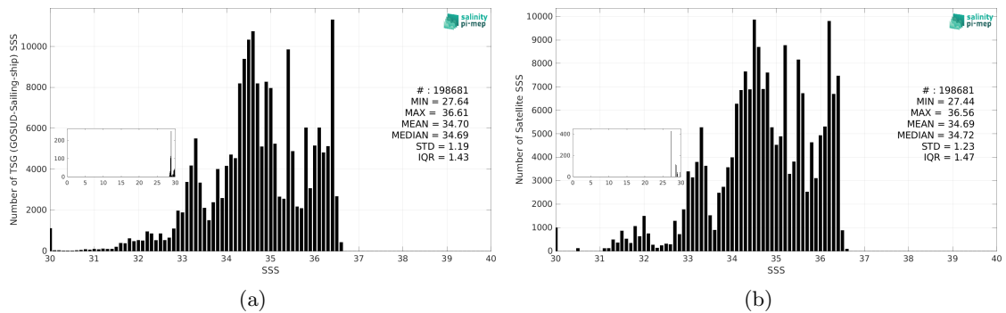
Figure 3: Histograms of SSS from TSG (GOSUD-Sailing-ship) (a) and CCI SSS L4 Merged-OI v5.5 - 7-day running (ESA) (b) considering all match-up pairs per bins of 0.1 over the Pacific Ocean Pi-MEP region and for the full satellite product period.
