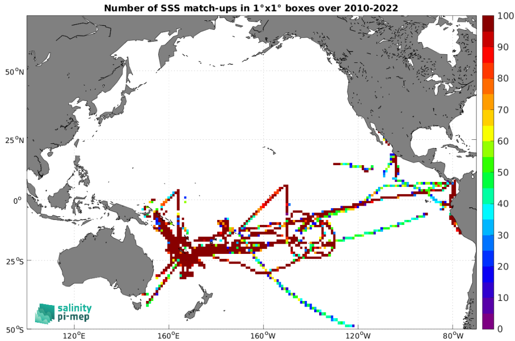
Figure 5: Number of SSS match-ups between TSG (GOSUD-Research-vessel) SSS and the CCI SSS L4 Merged-OI v5.5 - 7-day running (ESA) SSS product for the Pacific Ocean Pi-MEP region over 1^\circ \times 1^\circ boxes and for the full satellite product period.
