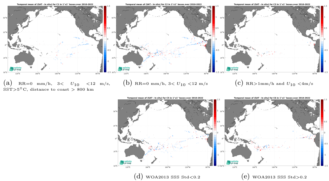
Figure 14: Temporal mean gridded over spatial boxes of size 1^\circ \times 1^\circ of \Delta SSS (CCI SSS L4 Merged-OI v5.5 - 7-day running (ESA) - TSG (GOSUD-Research-vessel)) for 5 different subdatasets corresponding to:RR=0 mm/h, 3 < U_{10} < 12 m/s, SST >5^\circ\text{C} , distance to coast > 800 km (a), RR=0 mm/h, 3 < U_{10} < 12 m/s (b), RR >1 mm/h and U_{10} < 4 m/s (c), WOA2013 SSS Std <0.2 (d), WOA2013 SSS Std >0.2 (e).
