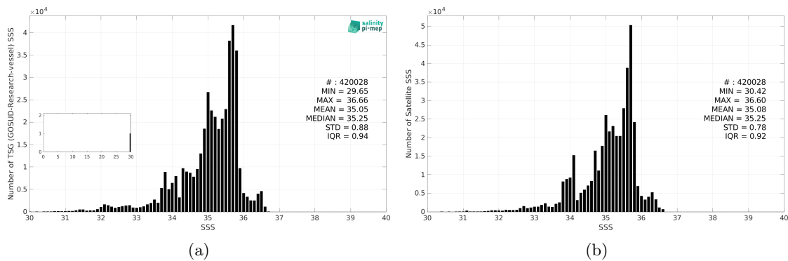
Figure 3: Histograms of SSS from TSG (GOSUD-Research-vessel) (a) and CCI SSS L4 Merged-OI v5.5 - 7-day running (ESA) (b) considering all match-up pairs per bins of 0.1 over the Pacific Ocean Pi-MEP region and for the full satellite product period.
