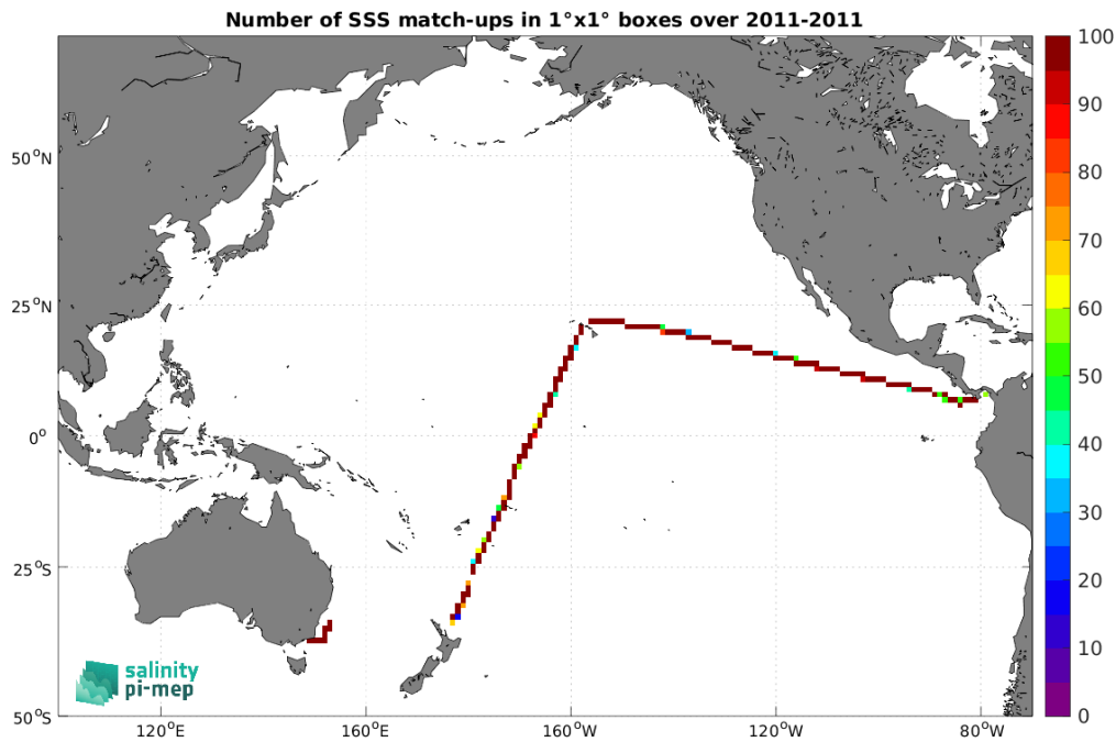
Figure 5: Number of SSS match-ups between TSG (CSIC-UTM) SSS and the CCI SSS L4 Merged-OI v5.5 - 7-day running (ESA) SSS product for the Pacific Ocean Pi-MEP region over 1^\circ \times 1^\circ boxes and for the full satellite product period.
