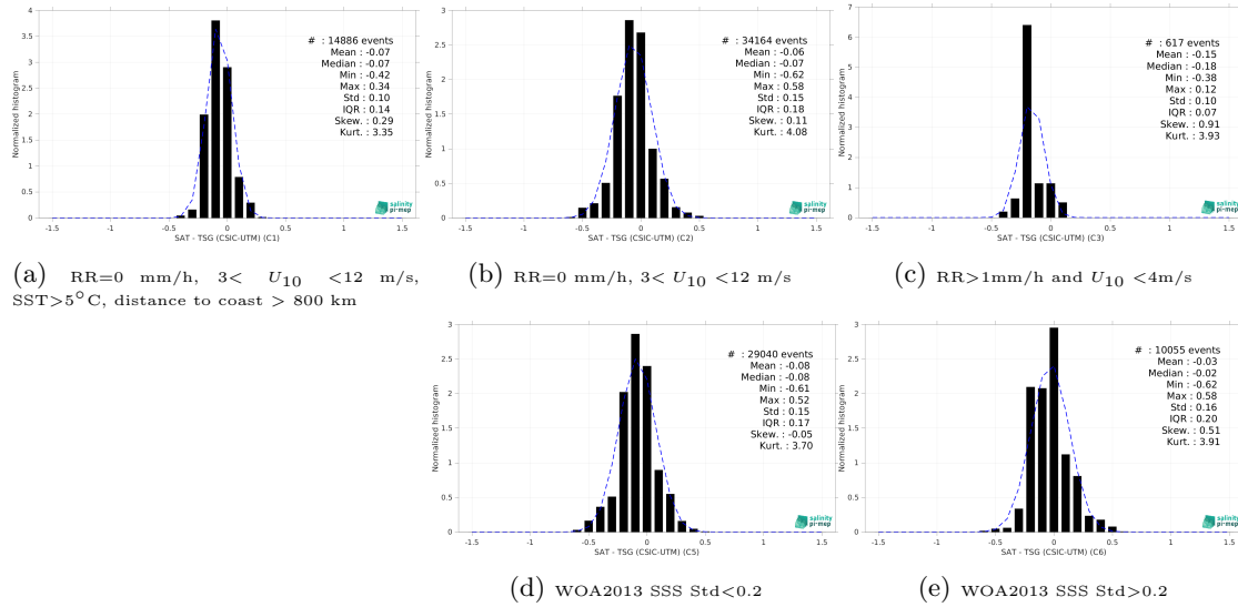
Figure 15: Normalized histogram of \Delta\text{SSS} (CCI SSS L4 Merged-OI v5.5 - 7-day running (ESA) - TSG (CSIC-UTM)) for 5 different subdatasets corresponding to: RR=0 mm/h, 3 < U_{10} < 12 m/s, SST>5°C, distance to coast > 800 km (a), RR=0 mm/h, 3 < U_{10} < 12 m/s (b), RR>1mm/h and U_{10} < 4 m/s (c), WOA2013 SSS Std<0.2 (d), WOA2013 SSS Std>0.2 (e).
