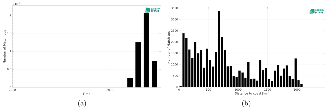
Figure 2: Number of match-ups between TSG (CSIC-UTM) and CCI SSS L4 Merged-OI v5.5 - 7-day running (ESA) SSS as a function of time (a) and as function of the distance to coast (b) over the Pacific Ocean Pi-MEP region and for the full satellite product period.
