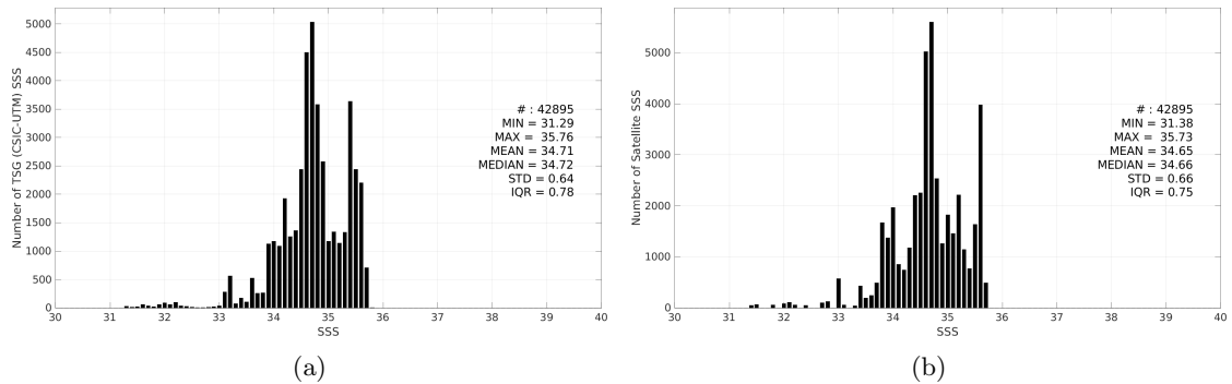
Figure 3: Histograms of SSS from TSG (CSIC-UTM) (a) and CCI SSS L4 Merged-OI v5.5 - 7-day running (ESA) (b) considering all match-up pairs per bins of 0.1 over the Pacific Ocean Pi-MEP region and for the full satellite product period.
