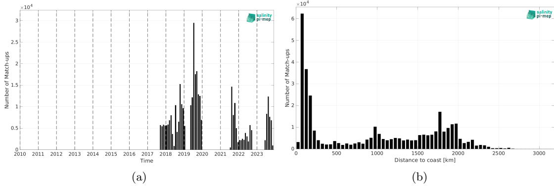
Figure 2: Number of match-ups between Saildrone and CCI SSS L4 Merged-OI v5.5 - 7-day running (ESA) SSS as a function of time (a) and as function of the distance to coast (b) over the Pacific Ocean Pi-MEP region and for the full satellite product period.
