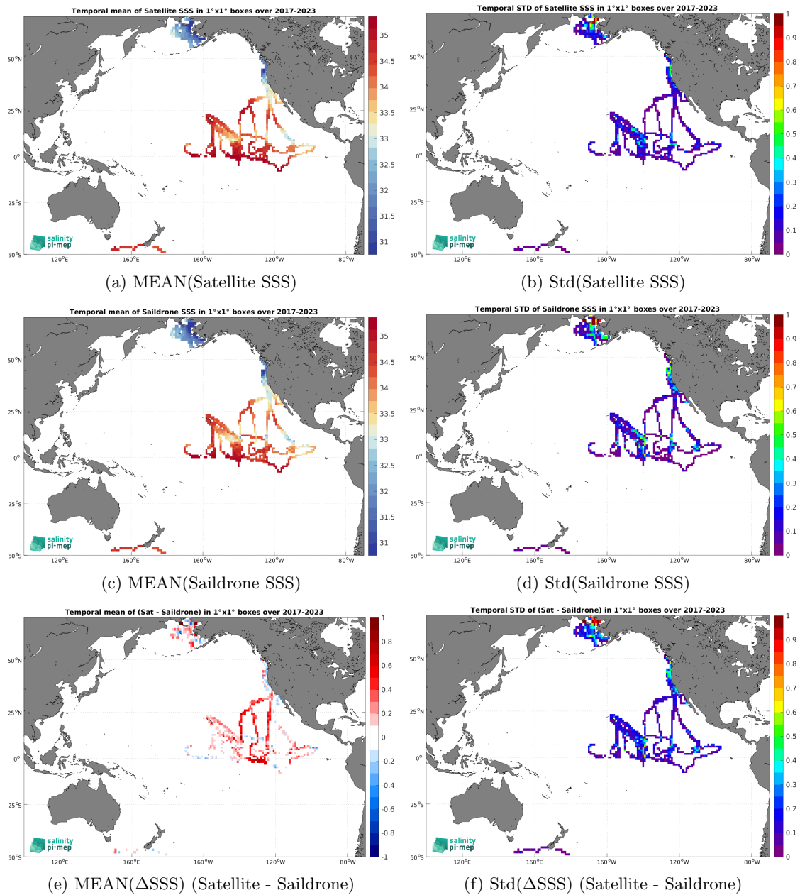
Figure 7: Temporal mean (left) and Std (right) of SSS from CCI SSS L4 Merged-OI v5.5 - 7-day running (ESA) (top), Saildrone (middle), and of \Delta SSS (Satellite - Saildrone). Only match-up pairs are used to generate these maps.
