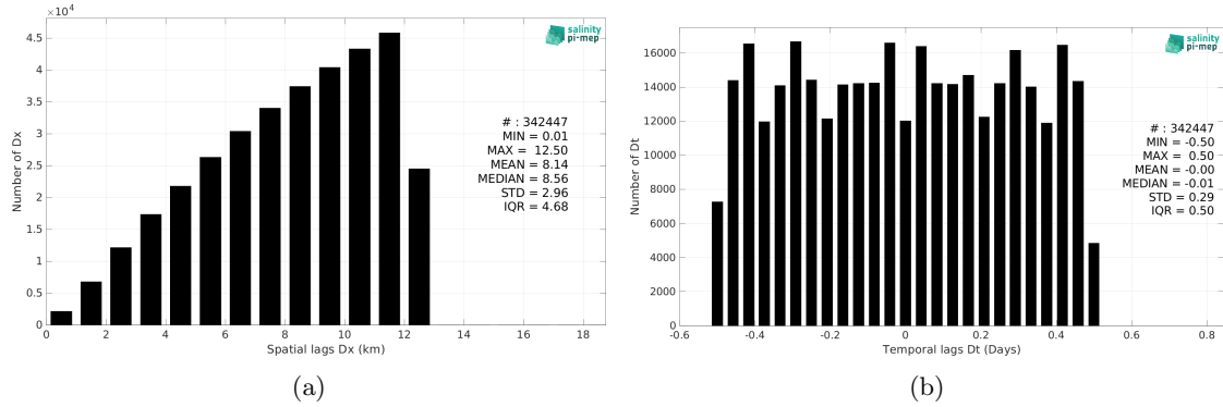
Figure 6: Histograms of the spatial (a) and temporal (b) lags between the location/time of the Sailability measurement and the date of the corresponding CCI SSS L4 Merged-OI v5.5 - 7-day running (ESA) SSS pixel.
