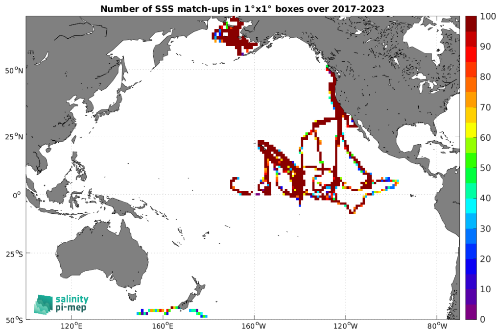
Figure 5: Number of SSS match-ups between Saildrone SSS and the CCI SSS L4 Merged-OI v5.5 - 7-day running (ESA) SSS product for the Pacific Ocean Pi-MEP region over 1^\circ \times 1^\circ boxes and for the full satellite product period.
