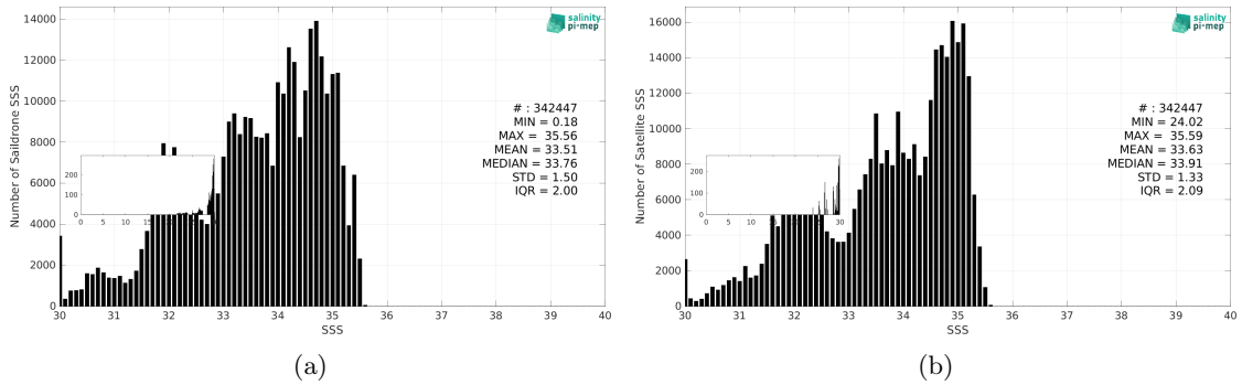
Figure 3: Histograms of SSS from Saildrone (a) and CCI SSS L4 Merged-OI v5.5 - 7-day running (ESA) (b) considering all match-up pairs per bins of 0.1 over the Pacific Ocean Pi-MEP region and for the full satellite product period.
