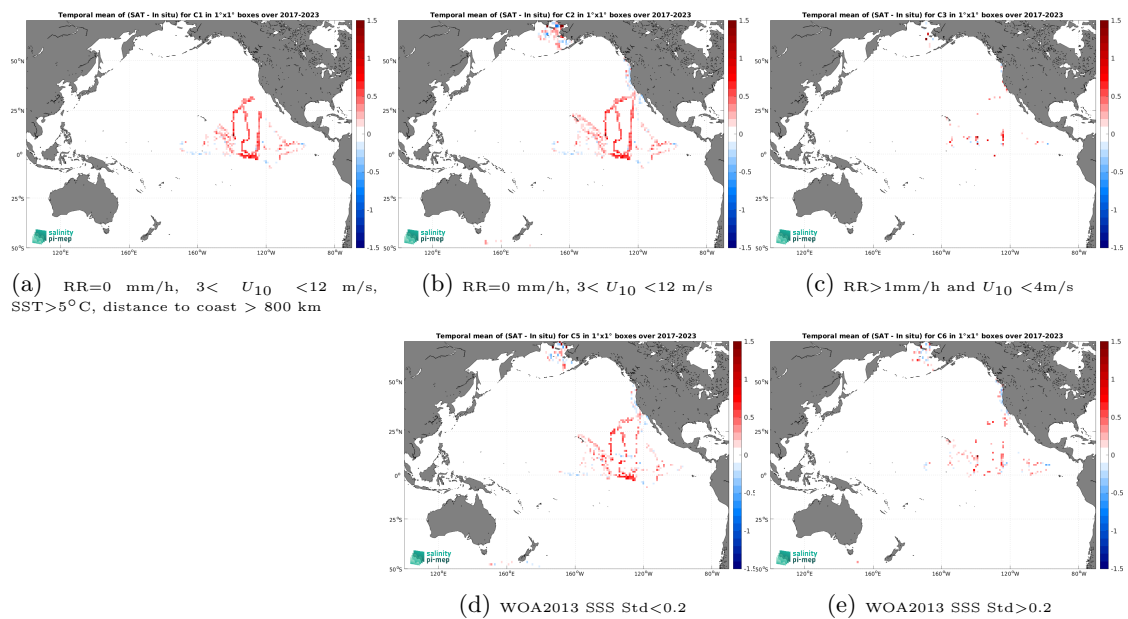
Figure 14: Temporal mean gridded over spatial boxes of size 1^\circ \times 1^\circ of \Delta\text{SSS} (CCI SSS L4 Merged-OI v5.5 - 7-day running (ESA) - Saildrone) for 5 different subdatasets corresponding to: RR=0 mm/h, 3 < U_{10} < 12 m/s, SST > 5^\circ\text{C} , distance to coast > 800 km (a), RR=0 mm/h, 3 < U_{10} < 12 m/s (b), RR > 1 mm/h and U_{10} < 4 m/s (c), WOA2013 SSS Std < 0.2 (d), WOA2013 SSS Std > 0.2 (e).
