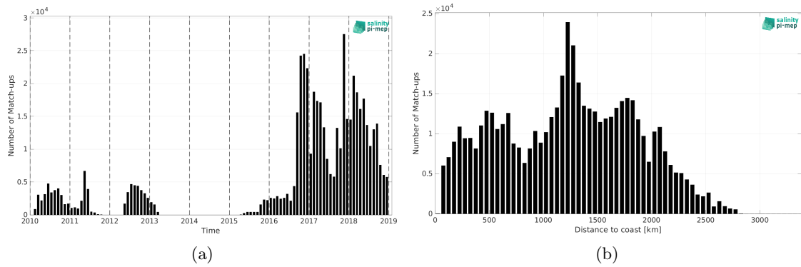
Figure 2: Number of match-ups between Surface drifters and CCI SSS L4 Merged-OI v5.5 - 7-day running (ESA) SSS as a function of time (a) and as function of the distance to coast (b) over the Pacific Ocean Pi-MEP region and for the full satellite product period.
