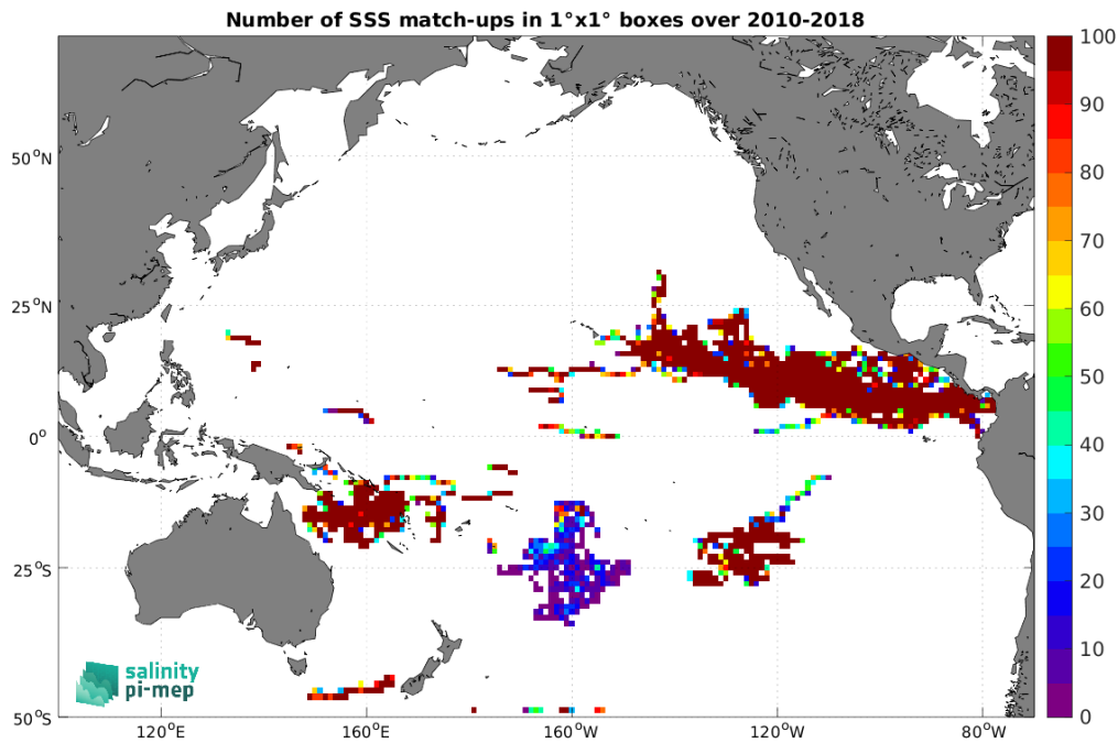
Figure 4: Number of SSS match-ups between Surface drifters SSS and the CCI SSS L4 Merged-OI v5.5 - 7-day running (ESA) SSS product for the Pacific Ocean Pi-MEP region over 1^\circ \times 1^\circ boxes and for the full satellite product period.
