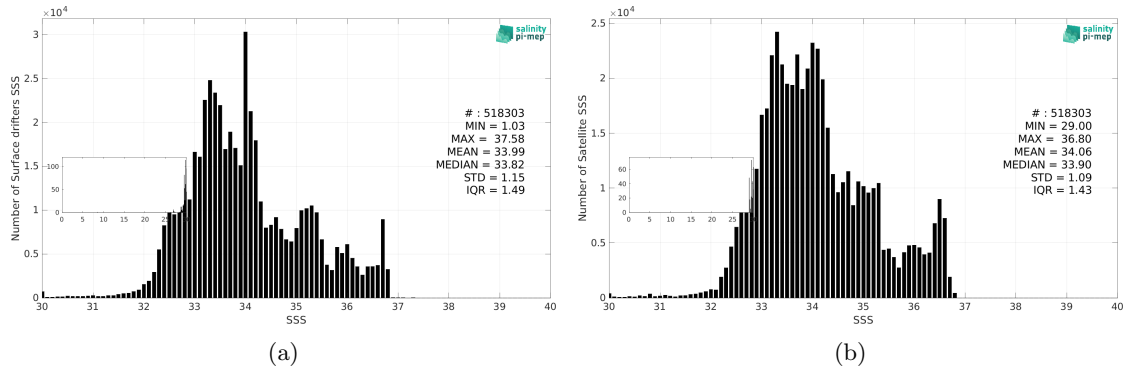
Figure 3: Histograms of SSS from Surface drifters (a) and CCI SSS L4 Merged-OI v5.5 - 7-day running (ESA) (b) considering all match-up pairs per bins of 0.1 over the Pacific Ocean Pi-MEP region and for the full satellite product period.
