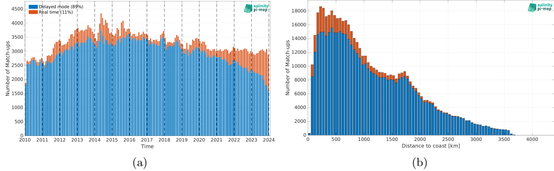
Figure 2: Number of match-ups between Argo and CCI SSS L4 Merged-OI v5.5 - 7-day running (ESA) SSS as a function of time (a) and as function of the distance to coast (b) over the Pacific Ocean Pi-MEP region and for the full satellite product period.
