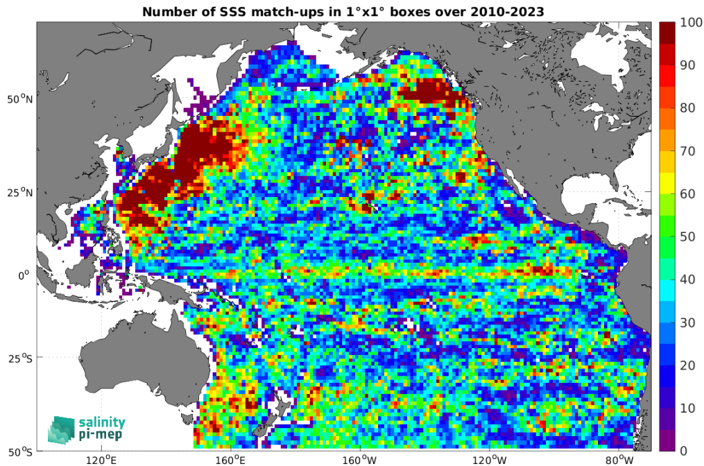
Figure 5: Number of SSS match-ups between Argo SSS and the CCI SSS L4 Merged-OI v5.5 - 7-day running (ESA) SSS product for the Pacific Ocean Pi-MEP region over 1^\circ \times 1^\circ boxes and for the full satellite product period.
