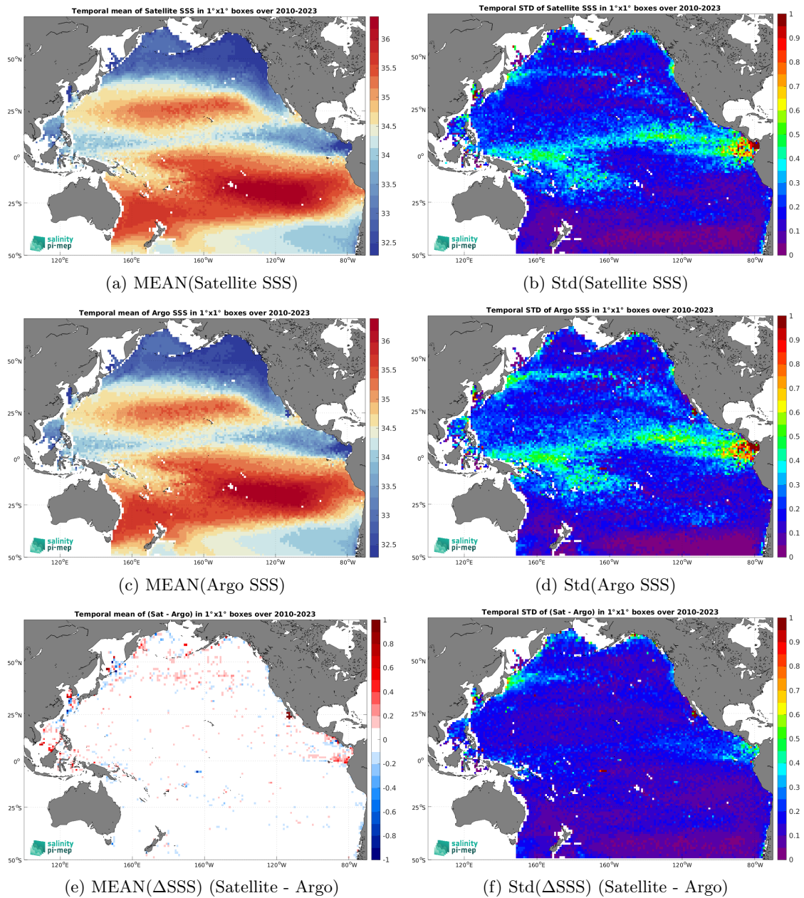
Figure 7: Temporal mean (left) and Std (right) of SSS from CCI SSS L4 Merged-OI v5.5 - 7-day running (ESA) (top), Argo (middle), and of \Delta SSS (Satellite - Argo). Only match-up pairs are used to generate these maps.
