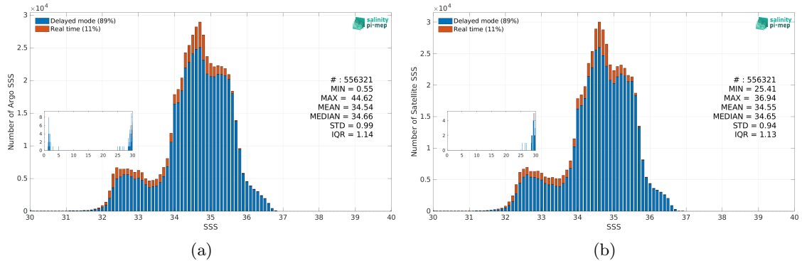
Figure 3: Histograms of SSS from Argo (a) and CCI SSS L4 Merged-OI v5.5 - 7-day running (ESA) (b) considering all match-up pairs per bins of 0.1 over the Pacific Ocean Pi-MEP region and for the full satellite product period.
