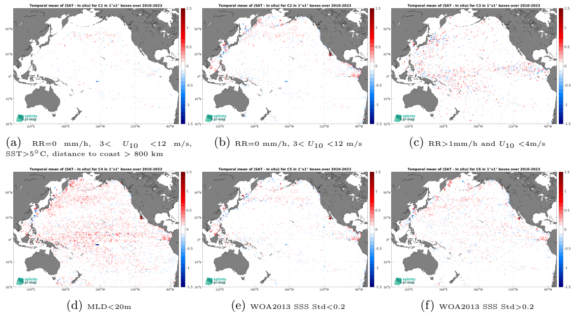
Figure 14: Temporal mean gridded over spatial boxes of size 1^\circ \times 1^\circ of \Delta SSS (CCI SSS L4 Merged-OI v5.5 - 7-day running (ESA) - Argo) for 6 different subdatasets corresponding to:RR=0 mm/h, 3 < U_{10} < 12 m/s, SST >5^\circ C, distance to coast > 800 km (a), RR=0 mm/h, 3 < U_{10} < 12 m/s (b), RR >1 mm/h and U_{10} < 4 m/s (c),MLD <20 m (d),WOA2013 SSS Std <0.2 (e),WOA2013 SSS Std >0.2 (f).
