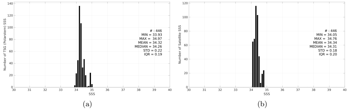
Figure 3: Histograms of SSS from TSG (Polarstern) (a) and CCI SSS L4 Merged-OI v5.5 - 30-day running (ESA) (b) considering all match-up pairs per bins of 0.1 over the Pacific Ocean Pi-MEP region and for the full satellite product period.
