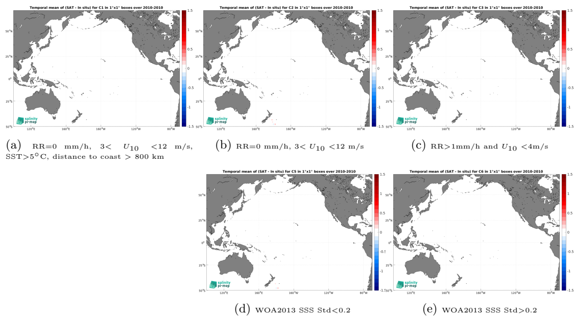
Figure 14: Temporal mean gridded over spatial boxes of size 1^\circ \times 1^\circ of \Delta SSS (CCI SSS L4 Merged-OI v5.5 - 30-day running (ESA) - TSG (Polarstern)) for 5 different subdatasets corresponding to:RR=0 mm/h, 3 < U_{10} < 12 m/s, SST >5^\circ C, distance to coast > 800 km (a), RR=0 mm/h, 3 < U_{10} < 12 m/s (b), RR >1 mm/h and U_{10} < 4 m/s (c), WOA2013 SSS Std <0.2 (d), WOA2013 SSS Std >0.2 (e).
