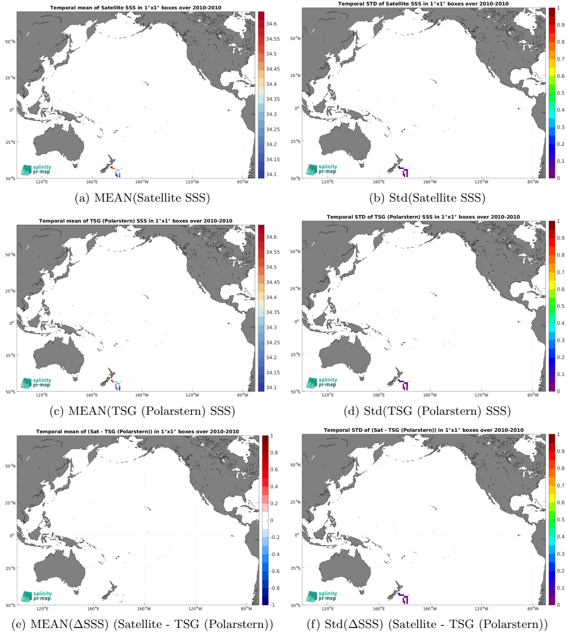
Figure 7: Temporal mean (left) and Std (right) of SSS from CCI SSS L4 Merged-OI v5.5 - 30-day running (ESA) (top), TSG (Polarstern) (middle), and of \Delta SSS (Satellite - TSG (Polarstern)). Only match-up pairs are used to generate these maps.
