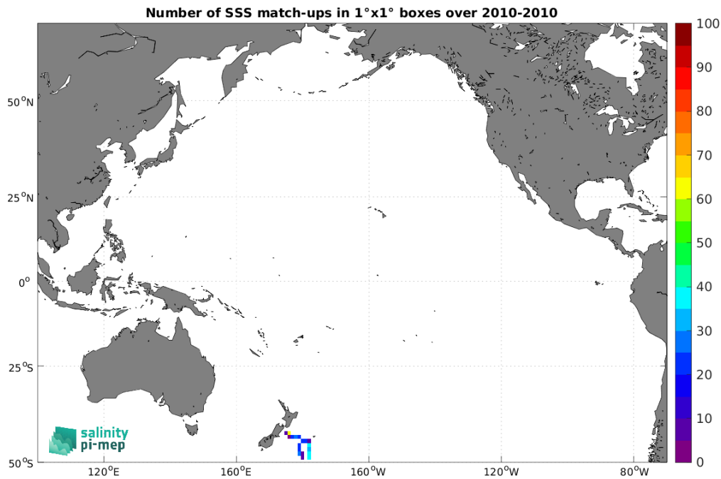
Figure 5: Number of SSS match-ups between TSG (Polarstern) SSS and the CCI SSS L4 Merged-OI v5.5 - 30-day running (ESA) SSS product for the Pacific Ocean Pi-MEP region over 1^\circ \times 1^\circ boxes and for the full satellite product period.
