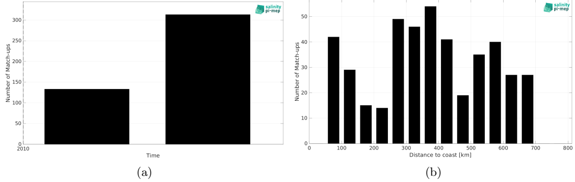
Figure 2: Number of match-ups between TSG (Polarstern) and CCI SSS L4 Merged-OI v5.5 - 30-day running (ESA) SSS as a function of time (a) and as function of the distance to coast (b) over the Pacific Ocean Pi-MEP region and for the full satellite product period.
