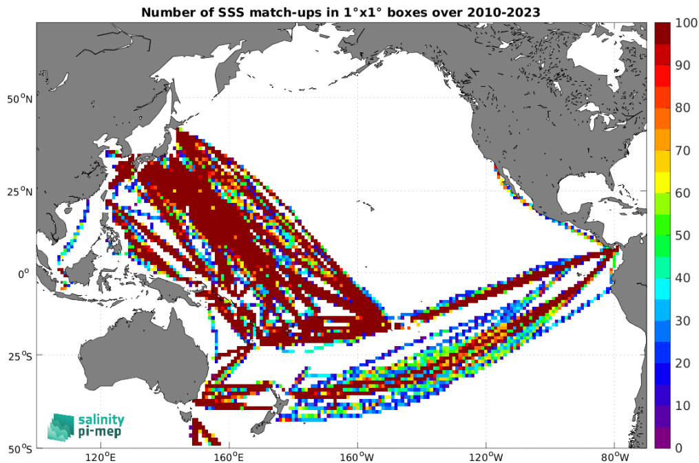
Figure 5: Number of SSS match-ups between TSG (LEGOS-DM) SSS and the CCI SSS L4 Merged-OI v5.5 - 30-day running (ESA) SSS product for the Pacific Ocean Pi-MEP region over 1^\circ \times 1^\circ boxes and for the full satellite product period.
