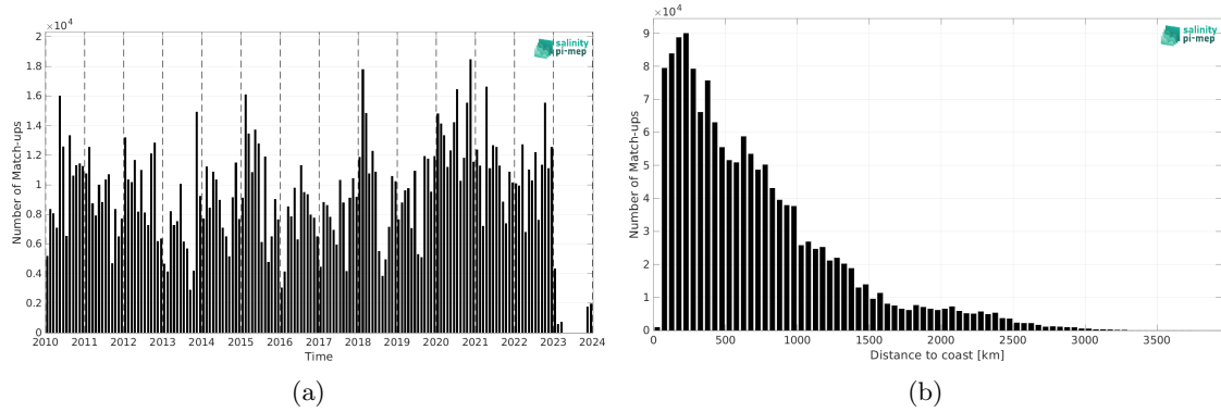
Figure 2: Number of match-ups between TSG (LEGOS-DM) and CCI SSS L4 Merged-OI v5.5 - 30-day running (ESA) SSS as a function of time (a) and as function of the distance to coast (b) over the Pacific Ocean Pi-MEP region and for the full satellite product period.
