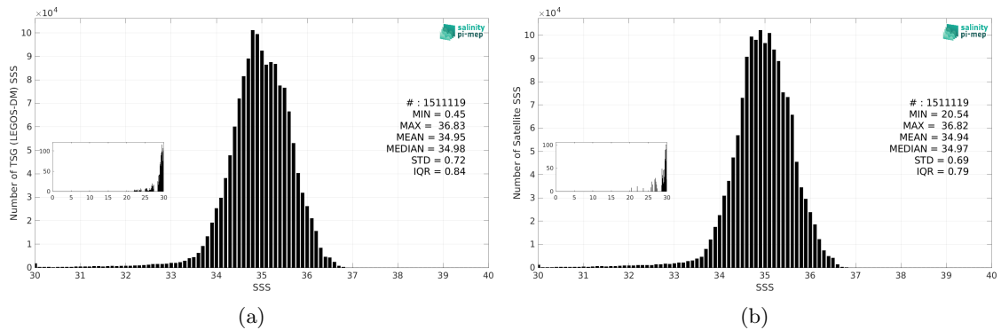
Figure 3: Histograms of SSS from TSG (LEGOS-DM) (a) and CCI SSS L4 Merged-OI v5.5 - 30-day running (ESA) (b) considering all match-up pairs per bins of 0.1 over the Pacific Ocean Pi-MEP region and for the full satellite product period.
