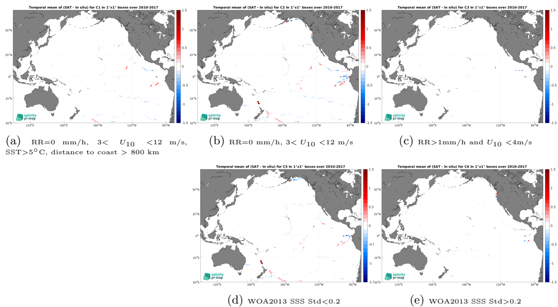
Figure 14: Temporal mean gridded over spatial boxes of size 1^\circ \times 1^\circ of \Delta SSS (CCI SSS L4 Merged-OI v5.5 - 30-day running (ESA) - TSG (GOSUD-Sailing-ship)) for 5 different subdatasets corresponding to:RR=0 mm/h, 3 < U_{10} < 12 m/s, SST >5^\circ C, distance to coast > 800 km (a), RR=0 mm/h, 3 < U_{10} < 12 m/s (b), RR >1 mm/h and U_{10} < 4 m/s (c), WOA2013 SSS Std <0.2 (d), WOA2013 SSS Std >0.2 (e).
