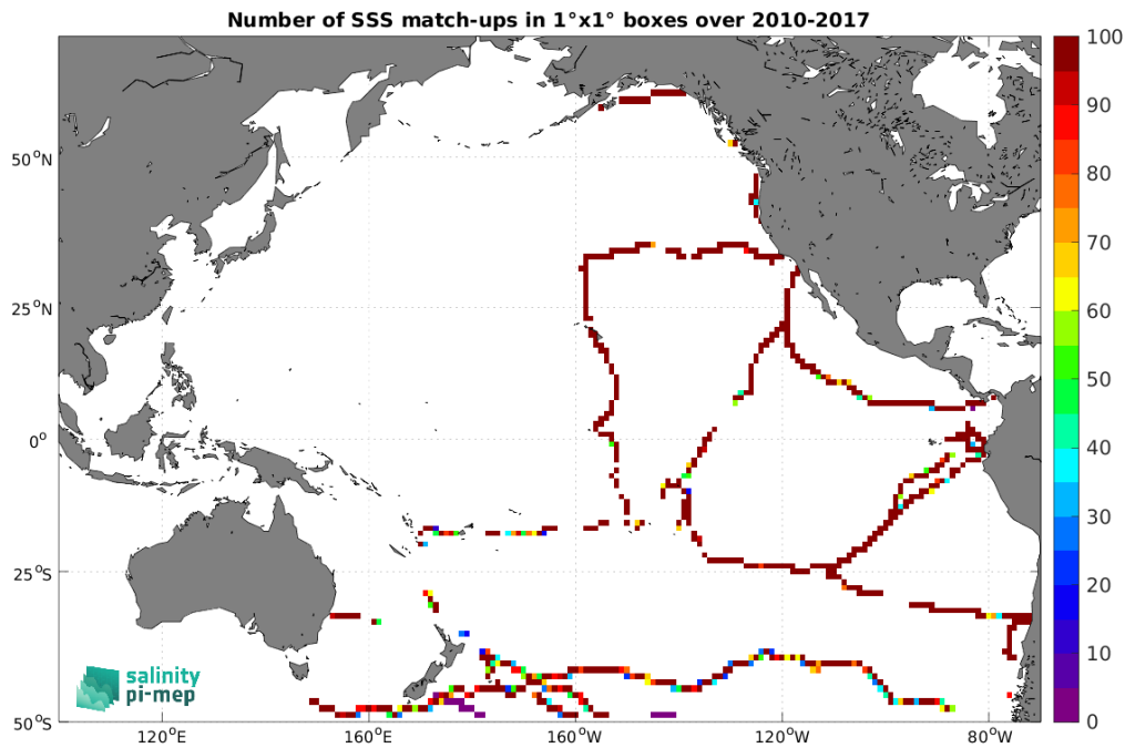
Figure 5: Number of SSS match-ups between TSG (GOSUD-Sailing-ship) SSS and the CCI SSS L4 Merged-OI v5.5 - 30-day running (ESA) SSS product for the Pacific Ocean Pi-MEP region over 1^\circ \times 1^\circ boxes and for the full satellite product period.
