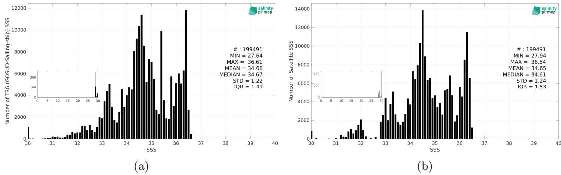
Figure 3: Histograms of SSS from TSG (GOSUD-Sailing-ship) (a) and CCI SSS L4 Merged-OI v5.5 - 30-day running (ESA) (b) considering all match-up pairs per bins of 0.1 over the Pacific Ocean Pi-MEP region and for the full satellite product period.
