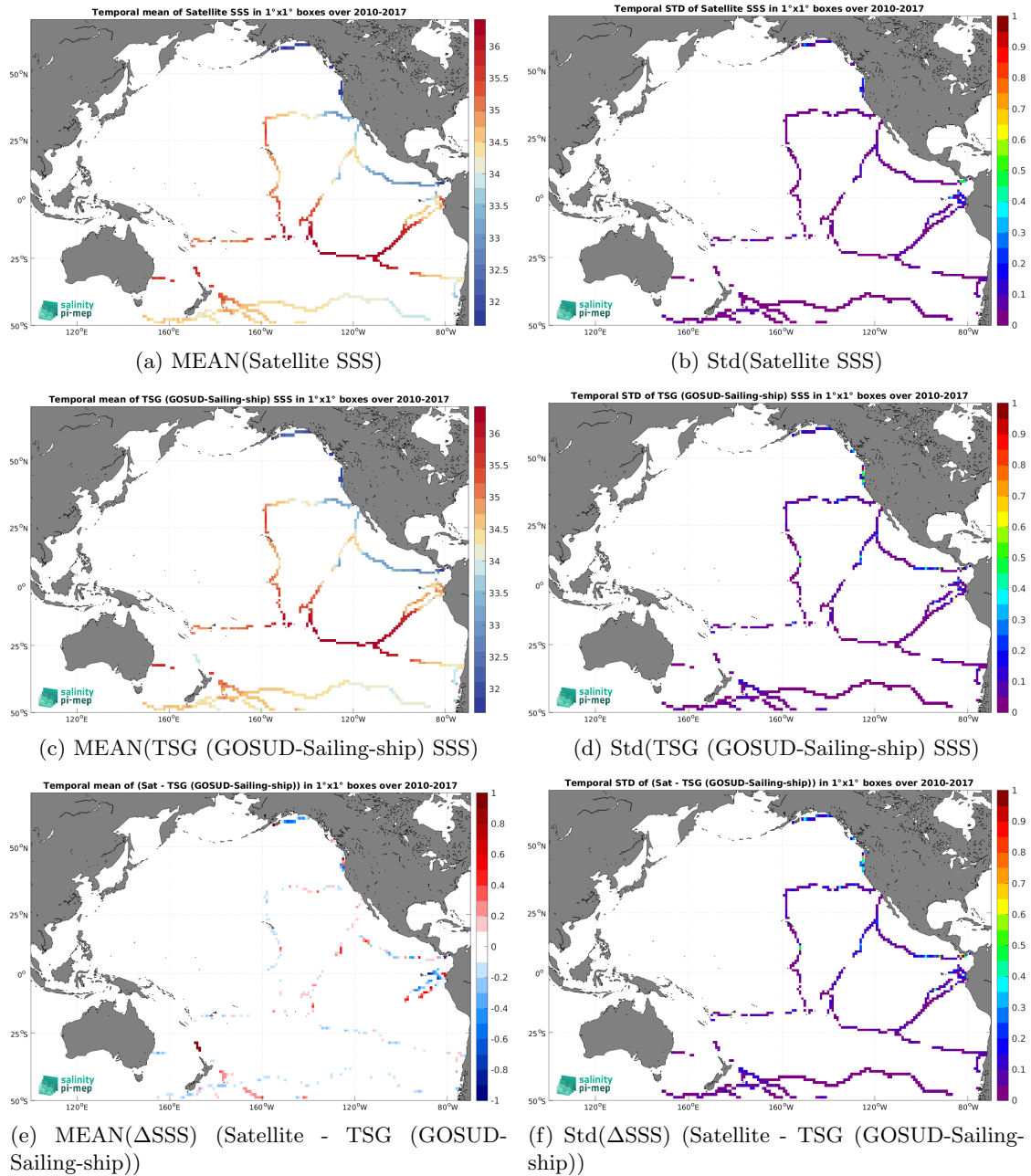
Figure 7: Temporal mean (left) and Std (right) of SSS from CCI SSS L4 Merged-OI v5.5 - 30-day running (ESA) (top), TSG (GOSUD-Sailing-ship) (middle), and of \Delta SSS (Satellite - TSG (GOSUD-Sailing-ship)). Only match-up pairs are used to generate these maps.
