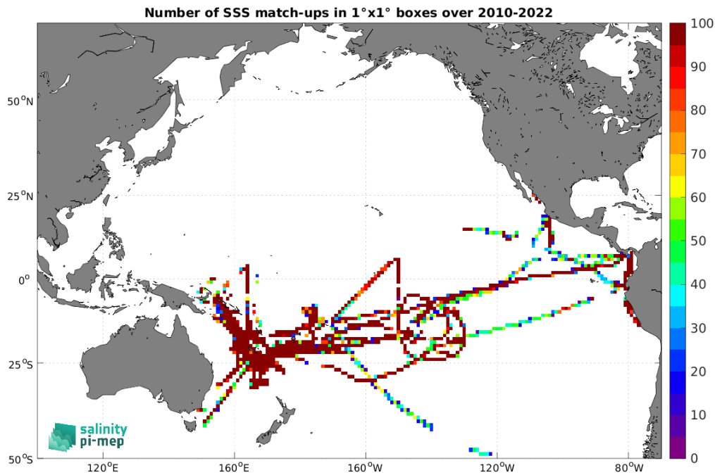
Figure 5: Number of SSS match-ups between TSG (GOSUD-Research-vessel) SSS and the CCI SSS L4 Merged-OI v5.5 - 30-day running (ESA) SSS product for the Pacific Ocean Pi-MEP region over 1^\circ \times 1^\circ boxes and for the full satellite product period.
