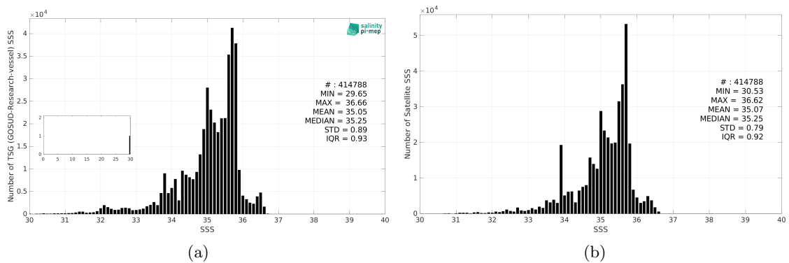
Figure 3: Histograms of SSS from TSG (GOSUD-Research-vessel) (a) and CCI SSS L4 Merged-OI v5.5 - 30-day running (ESA) (b) considering all match-up pairs per bins of 0.1 over the Pacific Ocean Pi-MEP region and for the full satellite product period.
