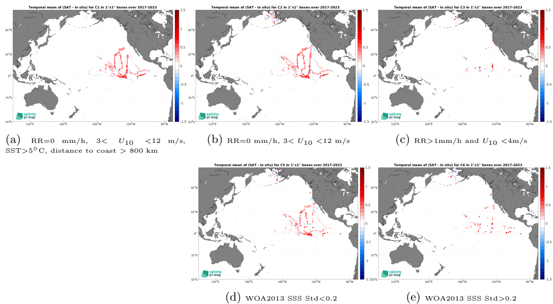
Figure 14: Temporal mean gridded over spatial boxes of size 1^\circ \times 1^\circ of \Delta SSS (CCI SSS L4 Merged-OI v5.5 - 30-day running (ESA) - Saildrone) for 5 different subdatasets corresponding to:RR=0 mm/h, 3 < U_{10} < 12 m/s, SST >5^\circ C, distance to coast > 800 km (a), RR=0 mm/h, 3 < U_{10} < 12 m/s (b), RR >1 mm/h and U_{10} < 4 m/s (c), WOA2013 SSS Std <0.2 (d), WOA2013 SSS Std >0.2 (e).
