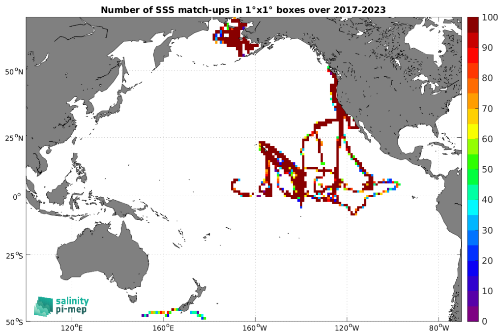
Figure 5: Number of SSS match-ups between Saildrone SSS and the CCI SSS L4 Merged-OI v5.5 - 30-day running (ESA) SSS product for the Pacific Ocean Pi-MEP region over 1^\circ \times 1^\circ boxes and for the full satellite product period.
