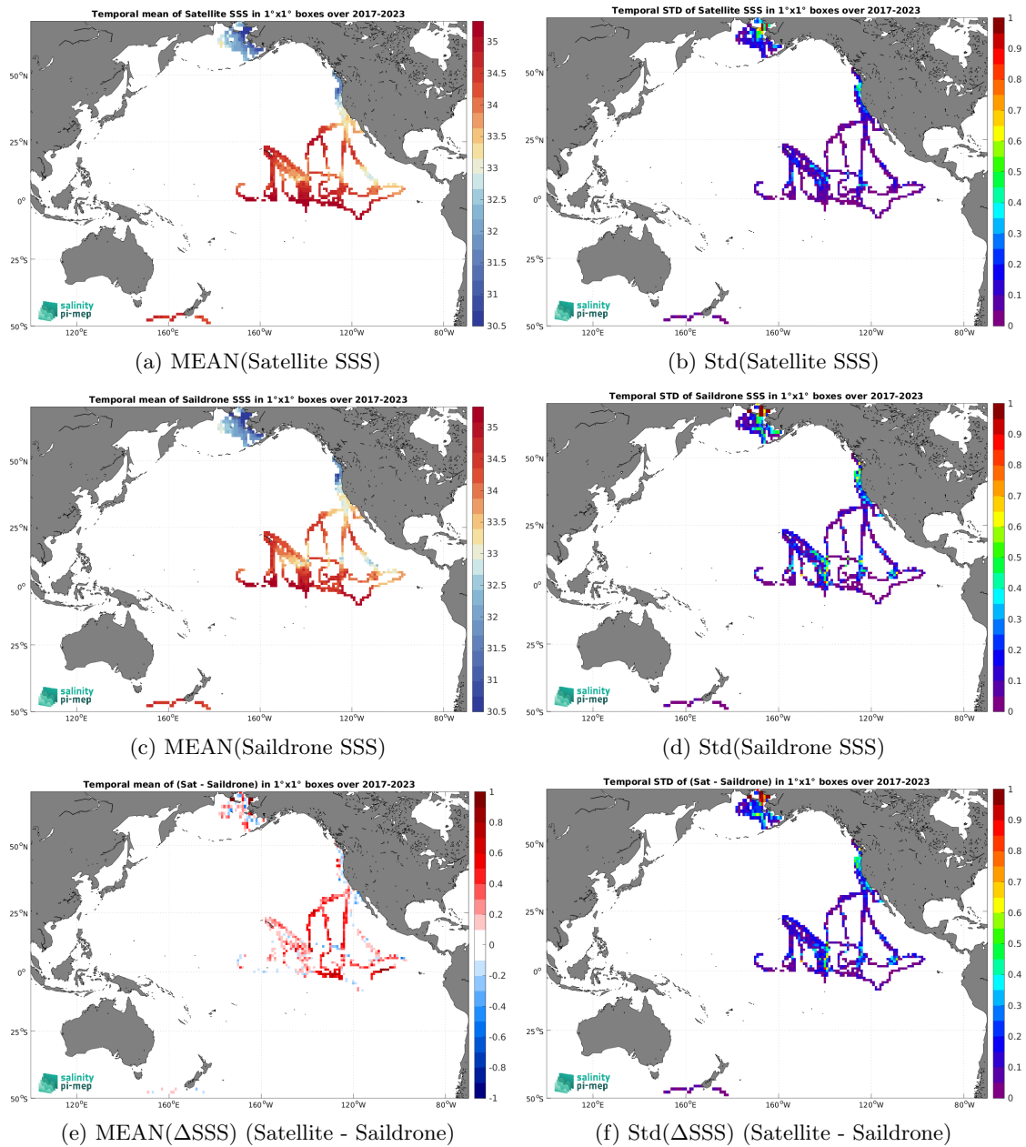
Figure 7: Temporal mean (left) and Std (right) of SSS from CCI SSS L4 Merged-OI v5.5 - 30-day running (ESA) (top), Saildrone (middle), and of \Delta SSS (Satellite - Saildrone). Only match-up pairs are used to generate these maps.
