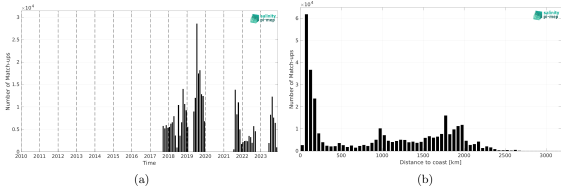
Figure 2: Number of match-ups between Saildrone and CCI SSS L4 Merged-OI v5.5 - 30-day running (ESA) SSS as a function of time (a) and as function of the distance to coast (b) over the Pacific Ocean Pi-MEP region and for the full satellite product period.
