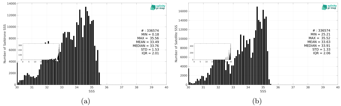
Figure 3: Histograms of SSS from Saildrone (a) and CCI SSS L4 Merged-OI v5.5 - 30-day running (ESA) (b) considering all match-up pairs per bins of 0.1 over the Pacific Ocean Pi-MEP region and for the full satellite product period.
