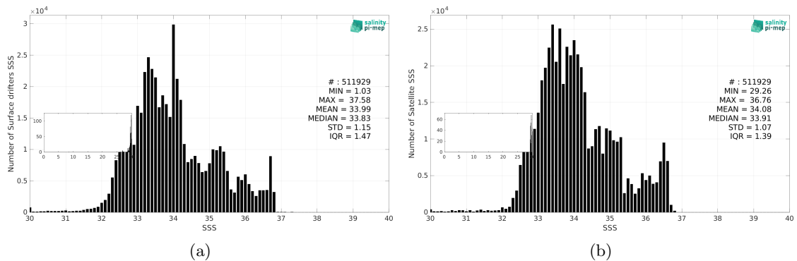
Figure 3: Histograms of SSS from Surface drifters (a) and CCI SSS L4 Merged-OI v5.5 - 30-day running (ESA) (b) considering all match-up pairs per bins of 0.1 over the Pacific Ocean Pi-MEP region and for the full satellite product period.
