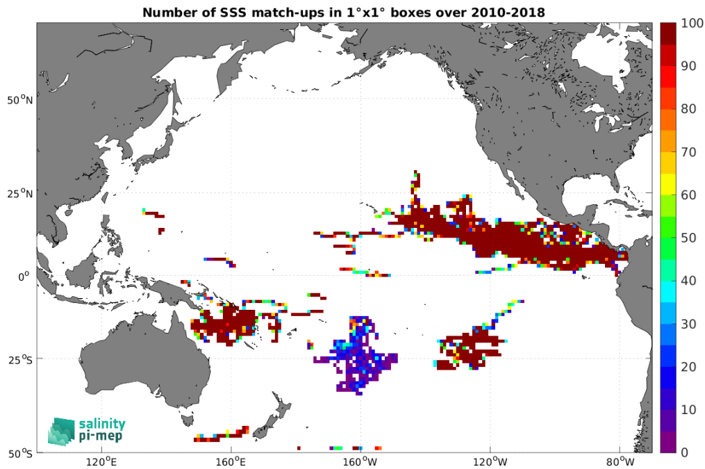
Figure 4: Number of SSS match-ups between Surface drifters SSS and the CCI SSS L4 Merged-OI v5.5 - 30-day running (ESA) SSS product for the Pacific Ocean Pi-MEP region over 1^\circ \times 1^\circ boxes and for the full satellite product period.
