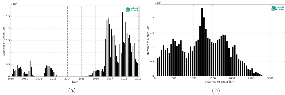
Figure 2: Number of match-ups between Surface drifters and CCI SSS L4 Merged-OI v5.5 - 30-day running (ESA) SSS as a function of time (a) and as function of the distance to coast (b) over the Pacific Ocean Pi-MEP region and for the full satellite product period.
