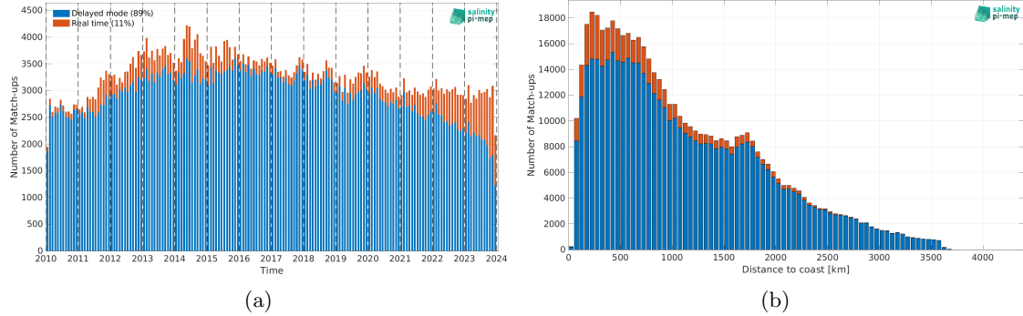
Figure 2: Number of match-ups between Argo and CCI SSS L4 Merged-OI v5.5 - 30-day running (ESA) SSS as a function of time (a) and as function of the distance to coast (b) over the Pacific Ocean Pi-MEP region and for the full satellite product period.
