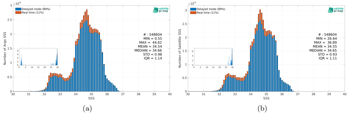
Figure 3: Histograms of SSS from Argo (a) and CCI SSS L4 Merged-OI v5.5 - 30-day running (ESA) (b) considering all match-up pairs per bins of 0.1 over the Pacific Ocean Pi-MEP region and for the full satellite product period.
