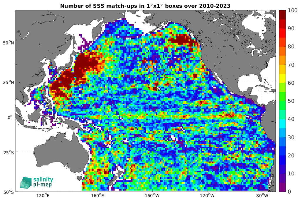
Figure 5: Number of SSS match-ups between Argo SSS and the CCI SSS L4 Merged-OI v5.5 - 30-day running (ESA) SSS product for the Pacific Ocean Pi-MEP region over 1^\circ \times 1^\circ boxes and for the full satellite product period.
