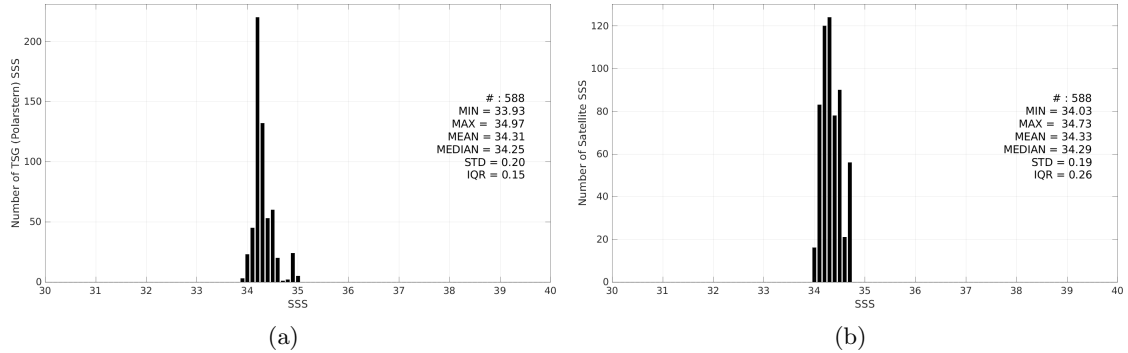
Figure 3: Histograms of SSS from TSG (Polarstern) (a) and CCI SSS L4 Merged-OI v4.41 - 7-day running (ESA) (b) considering all match-up pairs per bins of 0.1 over the Pacific Ocean Pi-MEP region and for the full satellite product period.
