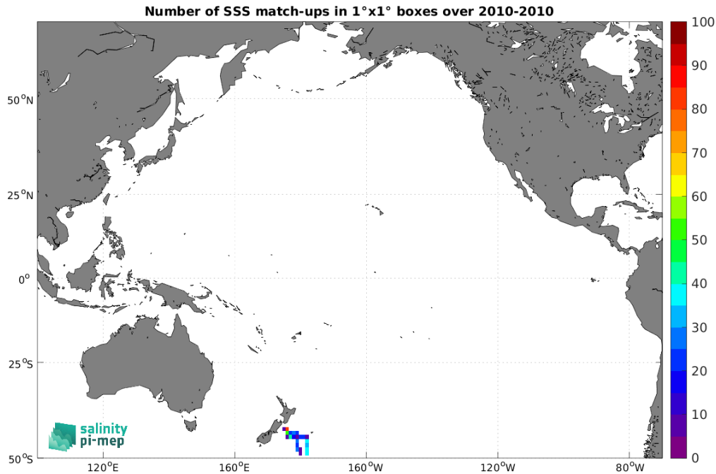
Figure 5: Number of SSS match-ups between TSG (Polarstern) SSS and the CCI SSS L4 Merged-OI v4.41 - 7-day running (ESA) SSS product for the Pacific Ocean Pi-MEP region over 1^\circ \times 1^\circ boxes and for the full satellite product period.
