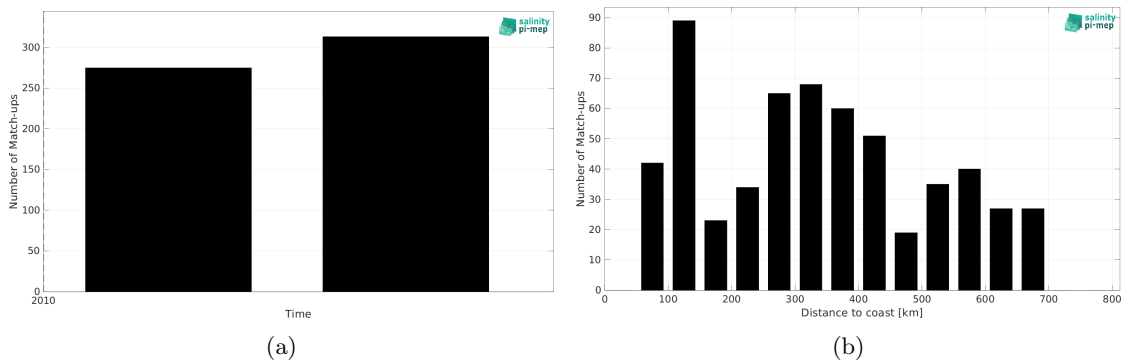
Figure 2: Number of match-ups between TSG (Polarstern) and CCI SSS L4 Merged-OI v4.41 - 7-day running (ESA) SSS as a function of time (a) and as function of the distance to coast (b) over the Pacific Ocean Pi-MEP region and for the full satellite product period.
