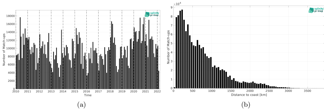
Figure 2: Number of match-ups between TSG (LEGOS-DM) and CCI SSS L4 Merged-OI v4.41 - 7-day running (ESA) SSS as a function of time (a) and as function of the distance to coast (b) over the Pacific Ocean Pi-MEP region and for the full satellite product period.
