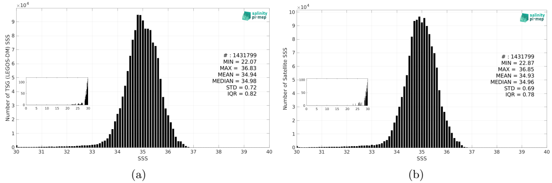
Figure 3: Histograms of SSS from TSG (LEGOS-DM) (a) and CCI SSS L4 Merged-OI v4.41 - 7-day running (ESA) (b) considering all match-up pairs per bins of 0.1 over the Pacific Ocean Pi-MEP region and for the full satellite product period.
