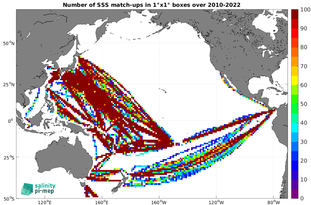
Figure 5: Number of SSS match-ups between TSG (LEGOS-DM) SSS and the CCI SSS L4 Merged-OI v4.41 - 7-day running (ESA) SSS product for the Pacific Ocean Pi-MEP region over 1^\circ \times 1^\circ boxes and for the full satellite product period.
