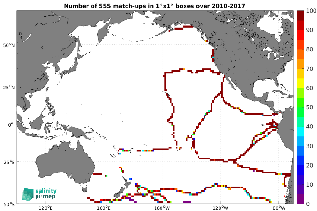
Figure 5: Number of SSS match-ups between TSG (GOSUD-Sailing-ship) SSS and the CCI SSS L4 Merged-OI v4.41 - 7-day running (ESA) SSS product for the Pacific Ocean Pi-MEP region over 1^\circ \times 1^\circ boxes and for the full satellite product period.
