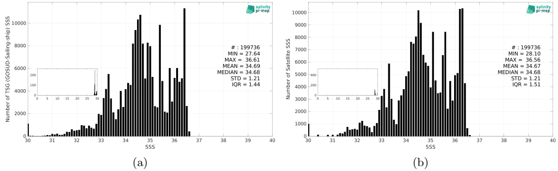
Figure 3: Histograms of SSS from TSG (GOSUD-Sailing-ship) (a) and CCI SSS L4 Merged-OI v4.41 - 7-day running (ESA) (b) considering all match-up pairs per bins of 0.1 over the Pacific Ocean Pi-MEP region and for the full satellite product period.
