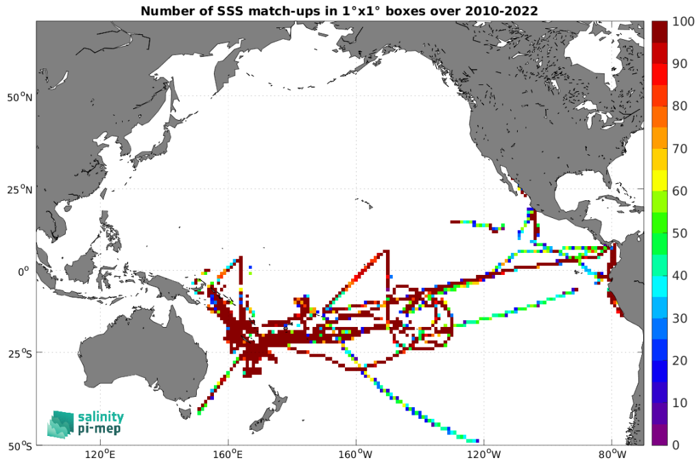
Figure 5: Number of SSS match-ups between TSG (GOSUD-Research-vessel) SSS and the CCI SSS L4 Merged-OI v4.41 - 7-day running (ESA) SSS product for the Pacific Ocean Pi-MEP region over 1^\circ \times 1^\circ boxes and for the full satellite product period.
