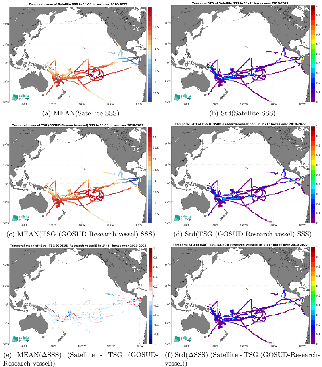
Figure 7: Temporal mean (left) and Std (right) of SSS from CCI SSS L4 Merged-OI v4.41 - 7-day running (ESA) (top), TSG (GOSUD-Research-vessel) (middle), and of \Delta SSS (Satellite - TSG (GOSUD-Research-vessel)). Only match-up pairs are used to generate these maps.
