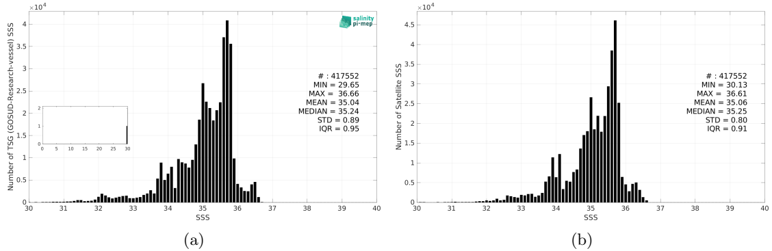
Figure 3: Histograms of SSS from TSG (GOSUD-Research-vessel) (a) and CCI SSS L4 Merged-OI v4.41 - 7-day running (ESA) (b) considering all match-up pairs per bins of 0.1 over the Pacific Ocean Pi-MEP region and for the full satellite product period.
