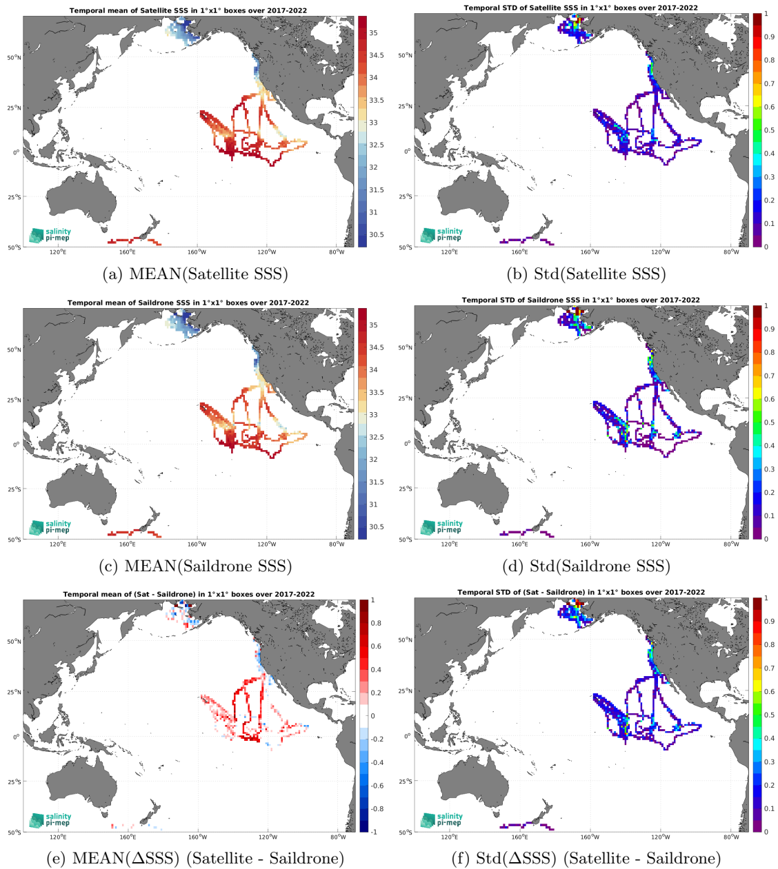
Figure 7: Temporal mean (left) and Std (right) of SSS from CCI SSS L4 Merged-OI v4.41 - 7-day running (ESA) (top), Saildrone (middle), and of \Delta SSS (Satellite - Saildrone). Only match-up pairs are used to generate these maps.
