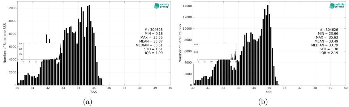
Figure 3: Histograms of SSS from Saildrone (a) and CCI SSS L4 Merged-OI v4.41 - 7-day running (ESA) (b) considering all match-up pairs per bins of 0.1 over the Pacific Ocean Pi-MEP region and for the full satellite product period.
