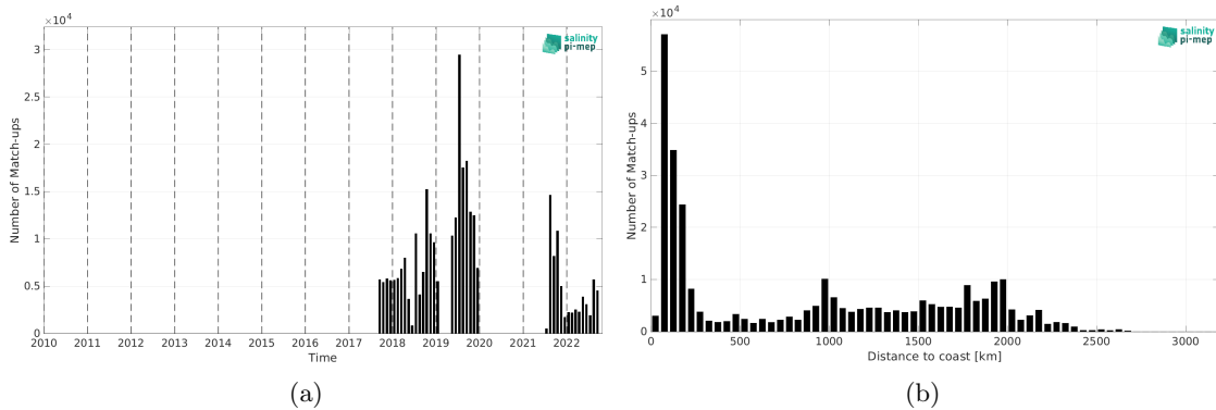
Figure 2: Number of match-ups between Saildrone and CCI SSS L4 Merged-OI v4.41 - 7-day running (ESA) SSS as a function of time (a) and as function of the distance to coast (b) over the Pacific Ocean Pi-MEP region and for the full satellite product period.
