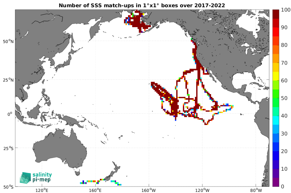
Figure 5: Number of SSS match-ups between Saildrone SSS and the CCI SSS L4 Merged-OI v4.41 - 7-day running (ESA) SSS product for the Pacific Ocean Pi-MEP region over 1^\circ \times 1^\circ boxes and for the full satellite product period.
