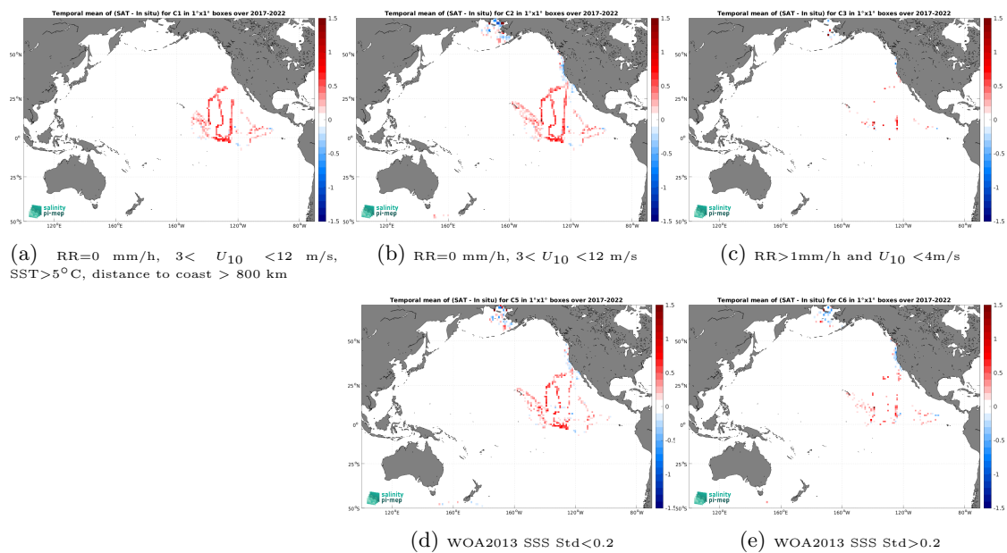
Figure 14: Temporal mean gridded over spatial boxes of size 1^\circ \times 1^\circ of \Delta SSS (CCI SSS L4 Merged-OI v4.41 - 7-day running (ESA) - Saildrone) for 5 different subdatasets corresponding to: RR=0 mm/h, 3 < U_{10} < 12 m/s, SST > 5^\circ\text{C} , distance to coast > 800 km (a), RR=0 mm/h, 3 < U_{10} < 12 m/s (b), RR > 1 mm/h and U_{10} < 4 m/s (c), WOA2013 SSS Std < 0.2 (d), WOA2013 SSS Std > 0.2 (e).
