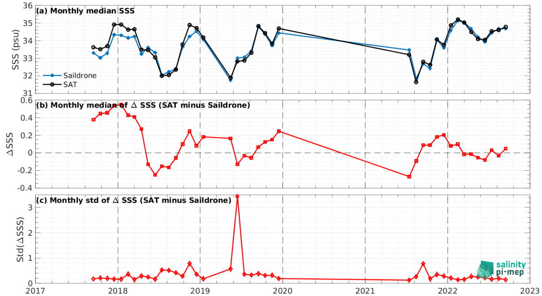
Figure 8: Time series of the monthly median SSS (top), median of \Delta\text{SSS} (Satellite - Saildrone) and Std of \Delta\text{SSS} (Satellite - Saildrone) over the Pacific Ocean Pi-MEP region considering all match-ups collected by the Pi-MEP.
