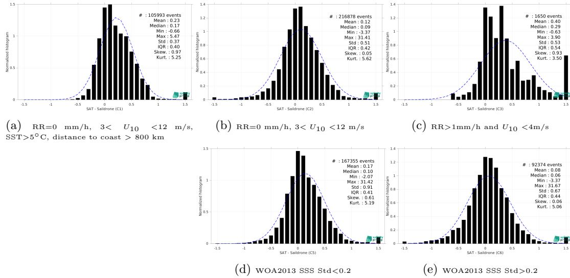
Figure 15: Normalized histogram of \Delta\text{SSS} (CCI SSS L4 Merged-OI v4.41 - 7-day running (ESA) - Saildrone) for 5 different subdatasets corresponding to: RR=0 mm/h, 3 < U_{10} < 12 m/s, SST > 5^\circ\text{C} , distance to coast > 800 km (a), RR=0 mm/h, 3 < U_{10} < 12 m/s (b), RR > 1 mm/h and U_{10} < 4 m/s (c), WOA2013 SSS Std < 0.2 (d), WOA2013 SSS Std > 0.2 (e).
