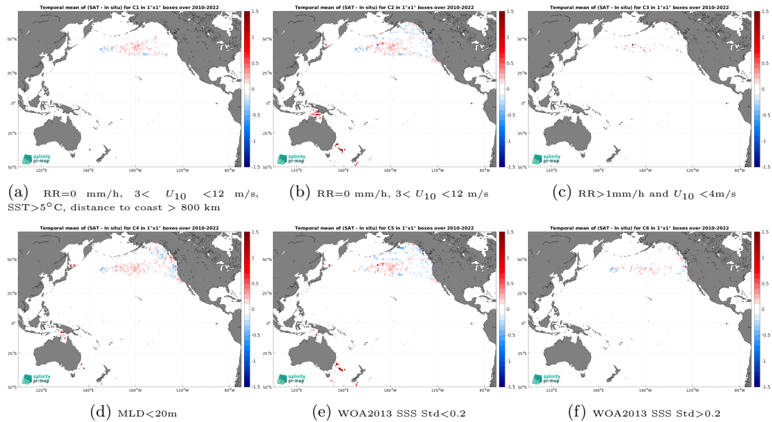
Figure 14: Temporal mean gridded over spatial boxes of size 1^\circ \times 1^\circ of \Delta\text{SSS} (CCI SSS L4 Merged-OI v4.41 - 7-day running (ESA) - Marine mammals) for 6 different subdatasets corresponding to:RR=0 mm/h, 3 < U_{10} < 12 m/s, SST>5°C, distance to coast > 800 km (a), RR=0 mm/h, 3 < U_{10} < 12 m/s (b), RR>1mm/h and U_{10} < 4 m/s (c),MLD<20m (d),WOA2013 SSS Std<0.2 (e),WOA2013 SSS Std>0.2 (f).
