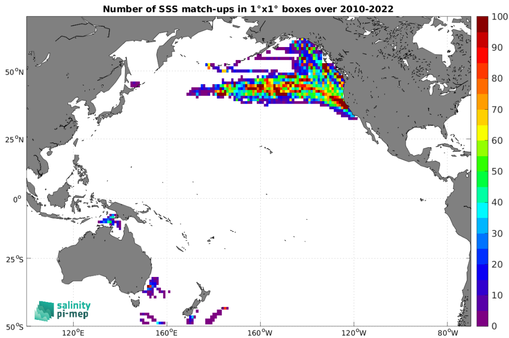
Figure 5: Number of SSS match-ups between Marine mammals SSS and the CCI SSS L4 Merged-OI v4.41 - 7-day running (ESA) SSS product for the Pacific Ocean Pi-MEP region over 1^\circ \times 1^\circ boxes and for the full satellite product period.
