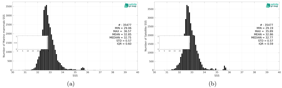
Figure 3: Histograms of SSS from Marine mammals (a) and CCI SSS L4 Merged-OI v4.41 - 7-day running (ESA) (b) considering all match-up pairs per bins of 0.1 over the Pacific Ocean Pi-MEP region and for the full satellite product period.
