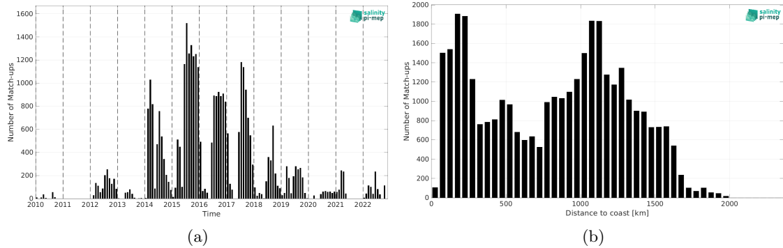
Figure 2: Number of match-ups between Marine mammals and CCI SSS L4 Merged-OI v4.41 - 7-day running (ESA) SSS as a function of time (a) and as function of the distance to coast (b) over the Pacific Ocean Pi-MEP region and for the full satellite product period.
