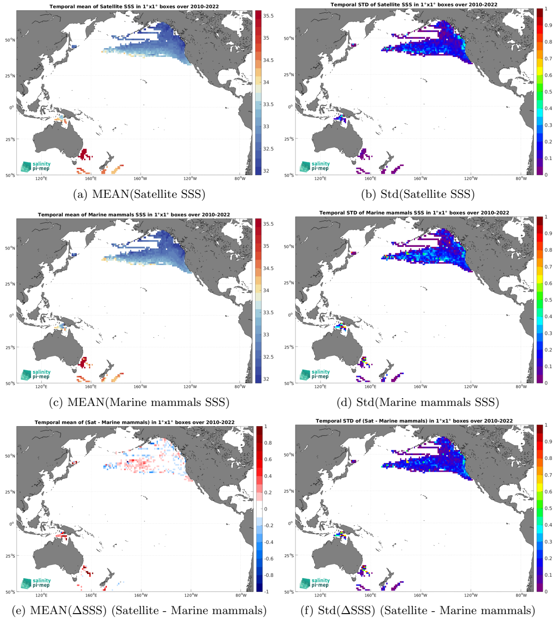
Figure 7: Temporal mean (left) and Std (right) of SSS from CCI SSS L4 Merged-OI v4.41 - 7-day running (ESA) (top), Marine mammals (middle), and of \Delta SSS (Satellite - Marine mammals). Only match-up pairs are used to generate these maps.
