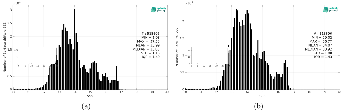
Figure 3: Histograms of SSS from Surface drifters (a) and CCI SSS L4 Merged-OI v4.41 - 7-day running (ESA) (b) considering all match-up pairs per bins of 0.1 over the Pacific Ocean Pi-MEP region and for the full satellite product period.
